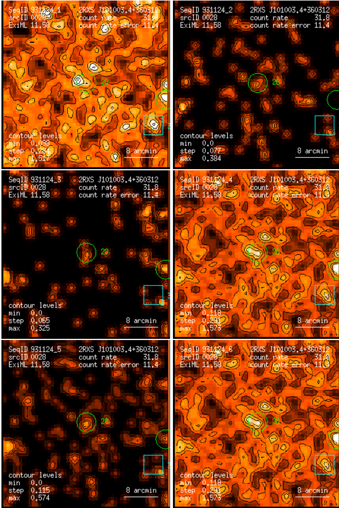
Figure 28: RASS 931124: detection 0028: band rate images, Gaussian filter: (1) PSPC channels 11 – 41, (2) 52 – 90, (3) 91 – 201, (4) 11 – 235, (5) 52 – 201, (6) 11 – 201. Broad band rates in counts/ks. Band rate contour levels in counts/ks/arcmin 2 .
