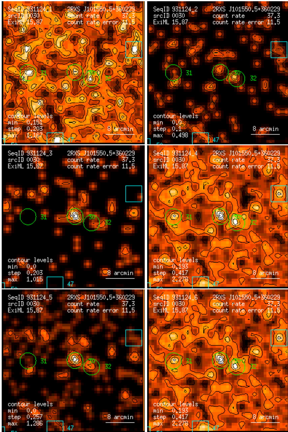
Figure 30: RASS 931124: detection 0030: band rate images, Gaussian filter: (1) PSPC channels 11 – 41, (2) 52 – 90, (3) 91 – 201, (4) 11 – 235, (5) 52 – 201, (6) 11 – 201. Broad band rates in counts/ks. Band rate contour levels in counts/ks/arcmin 2 .
