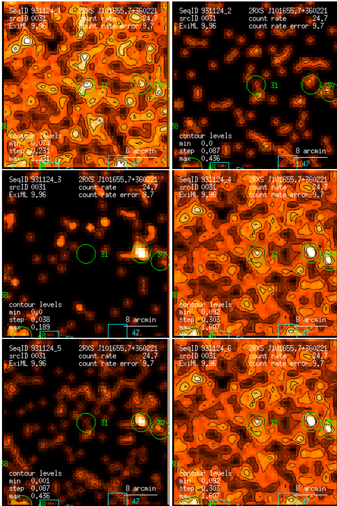
Figure 31: RASS 931124: detection 0031: band rate images, Gaussian filter: (1) PSPC channels 11 – 41, (2) 52 – 90, (3) 91 – 201, (4) 11 – 235, (5) 52 – 201, (6) 11 – 201. Broad band rates in counts/ks. Band rate contour levels in counts/ks/arcmin 2 .
