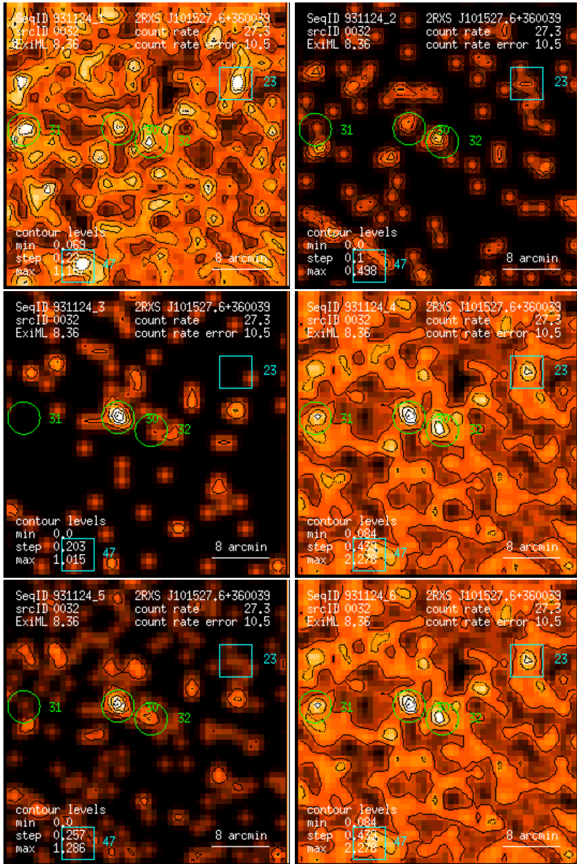
Figure 32: RASS 931124: detection 0032: band rate images, Gaussian filter: (1) PSPC channels 11 – 41, (2) 52 – 90, (3) 91 – 201, (4) 11 – 235, (5) 52 – 201, (6) 11 – 201. Broad band rates in counts/ks. Band rate contour levels in counts/ks/arcmin 2 .
