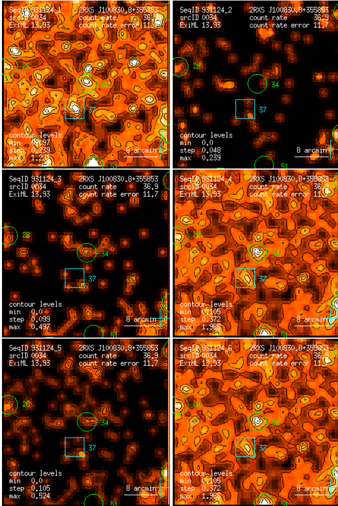
Figure 34: RASS 931124: detection 0034: band rate images, Gaussian filter: (1) PSPC channels 11 – 41, (2) 52 – 90, (3) 91 – 201, (4) 11 – 235, (5) 52 – 201, (6) 11 – 201. Broad band rates in counts/ks. Band rate contour levels in counts/ks/arcmin 2 .
