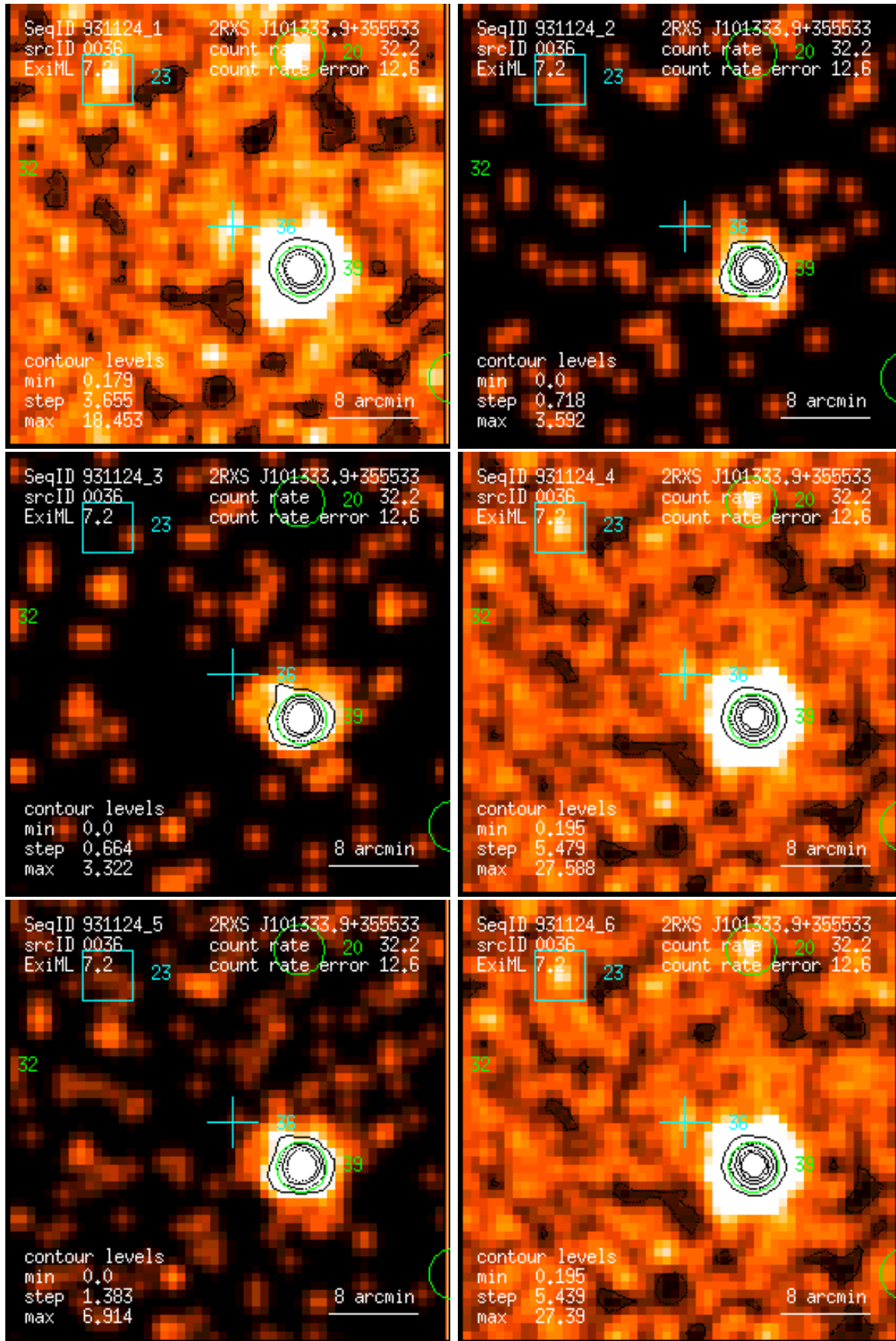
Figure 36: RASS 931124: detection 0036: band rate images, Gaussian filter: (1) PSPC channels 11 – 41, (2) 52 – 90, (3) 91 – 201, (4) 11 – 235, (5) 52 – 201, (6) 11 – 201. Broad band rates in counts/ks. Band rate contour levels in counts/ks/arcmin 2 .
