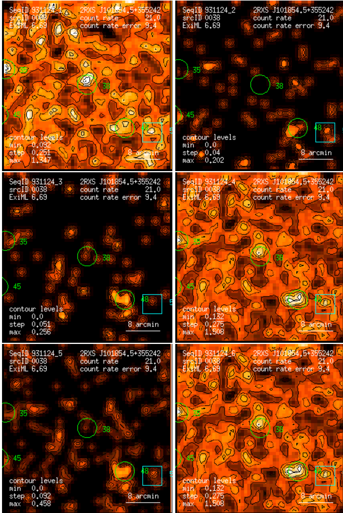
Figure 38: RASS 931124: detection 0038: band rate images, Gaussian filter: (1) PSPC channels 11 – 41, (2) 52 – 90, (3) 91 – 201, (4) 11 – 235, (5) 52 – 201, (6) 11 – 201. Broad band rates in counts/ks. Band rate contour levels in counts/ks/arcmin 2 .
