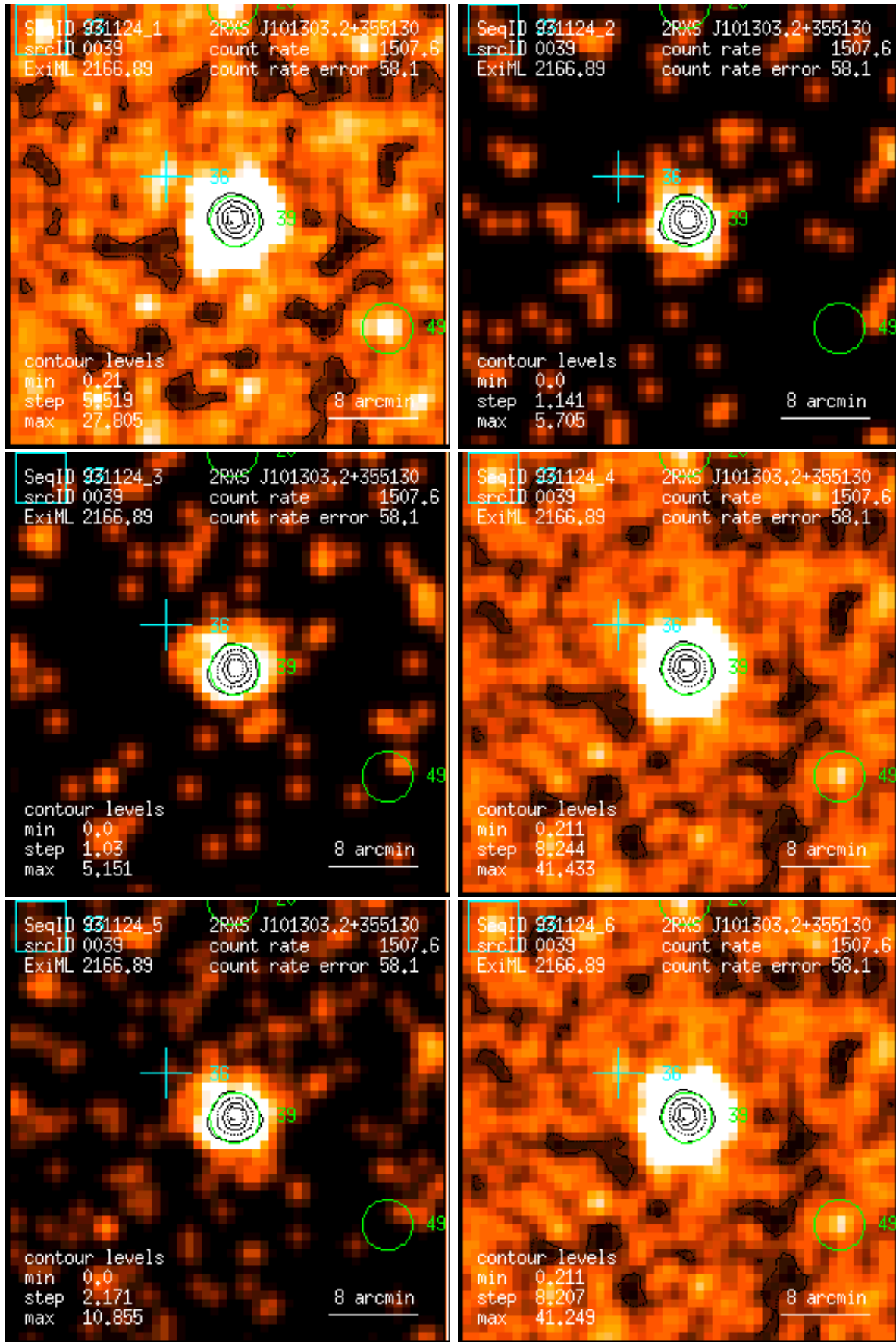
Figure 39: RASS 931124: detection 0039: band rate images, Gaussian filter: (1) PSPC channels 11 – 41, (2) 52 – 90, (3) 91 – 201, (4) 11 – 235, (5) 52 – 201, (6) 11 – 201. Broad band rates in counts/ks. Band rate contour levels in counts/ks/arcmin 2 .
