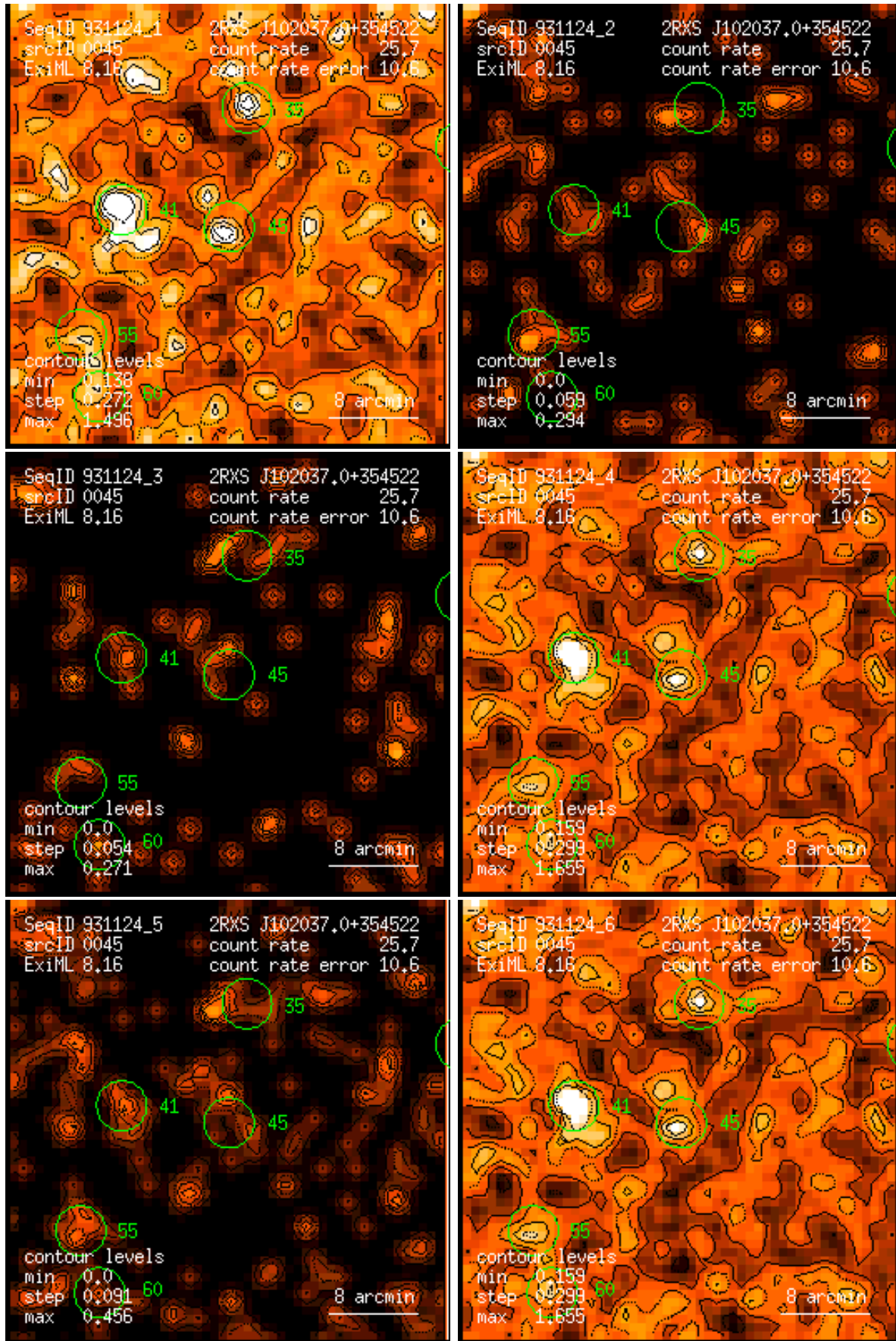
Figure 45: RASS 931124: detection 0045: band rate images, Gaussian filter: (1) PSPC channels 11 – 41, (2) 52 – 90, (3) 91 – 201, (4) 11 – 235, (5) 52 – 201, (6) 11 – 201. Broad band rates in counts/ks. Band rate contour levels in counts/ks/arcmin 2 .
