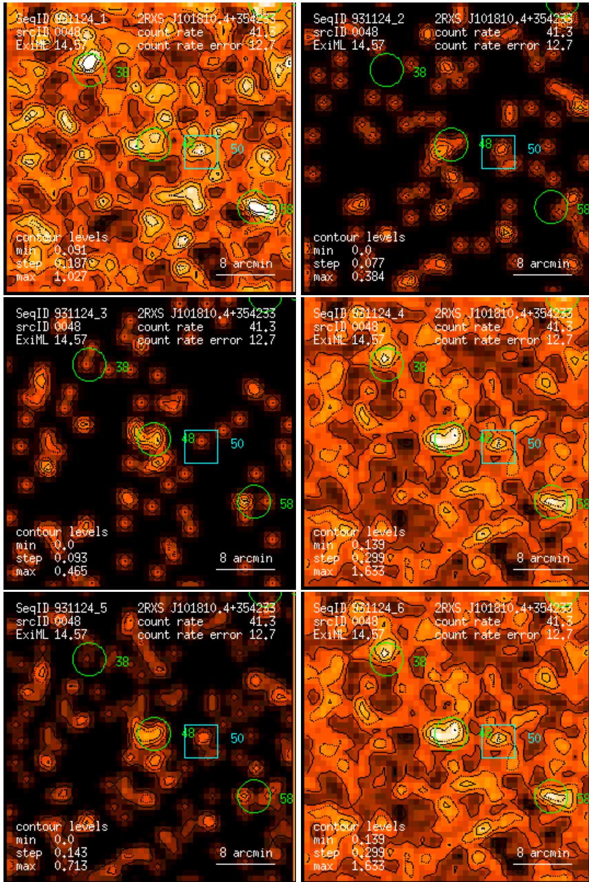
Figure 48: RASS 931124: detection 0048: band rate images, Gaussian filter: (1) PSPC channels 11 – 41, (2) 52 – 90, (3) 91 – 201, (4) 11 – 235, (5) 52 – 201, (6) 11 – 201. Broad band rates in counts/ks. Band rate contour levels in counts/ks/arcmin 2 .
