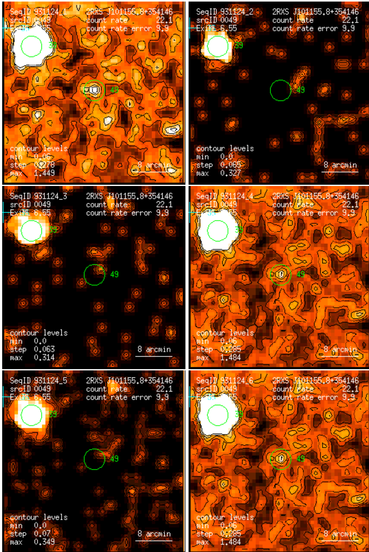
Figure 49: RASS 931124: detection 0049: band rate images, Gaussian filter: (1) PSPC channels 11 – 41, (2) 52 – 90, (3) 91 – 201, (4) 11 – 235, (5) 52 – 201, (6) 11 – 201. Broad band rates in counts/ks. Band rate contour levels in counts/ks/arcmin 2 .
