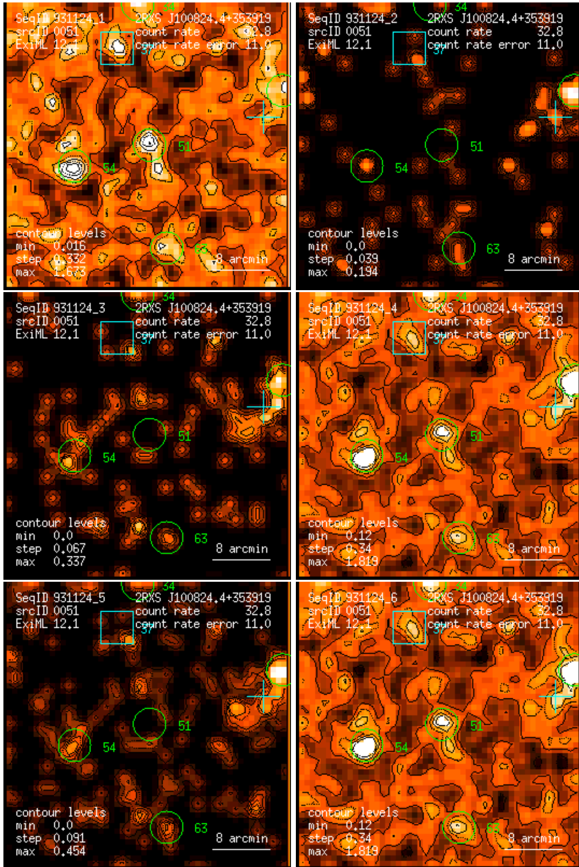
Figure 51: RASS 931124: detection 0051: band rate images, Gaussian filter: (1) PSPC channels 11 – 41, (2) 52 – 90, (3) 91 – 201, (4) 11 – 235, (5) 52 – 201, (6) 11 – 201. Broad band rates in counts/ks. Band rate contour levels in counts/ks/arcmin 2 .
