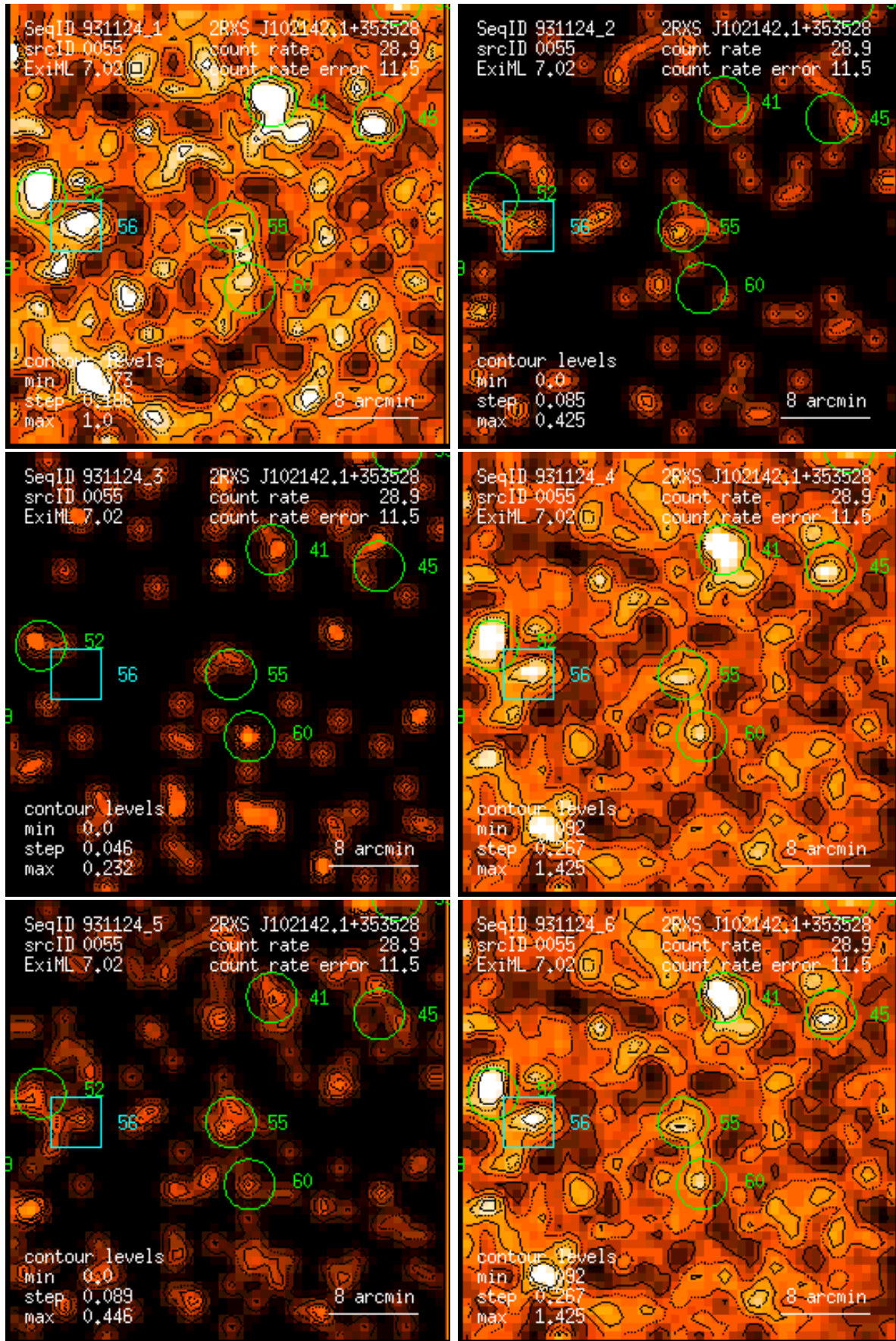
Figure 55: RASS 931124: detection 0055: band rate images, Gaussian filter: (1) PSPC channels 11 – 41, (2) 52 – 90, (3) 91 – 201, (4) 11 – 235, (5) 52 – 201, (6) 11 – 201. Broad band rates in counts/ks. Band rate contour levels in counts/ks/arcmin 2 .
