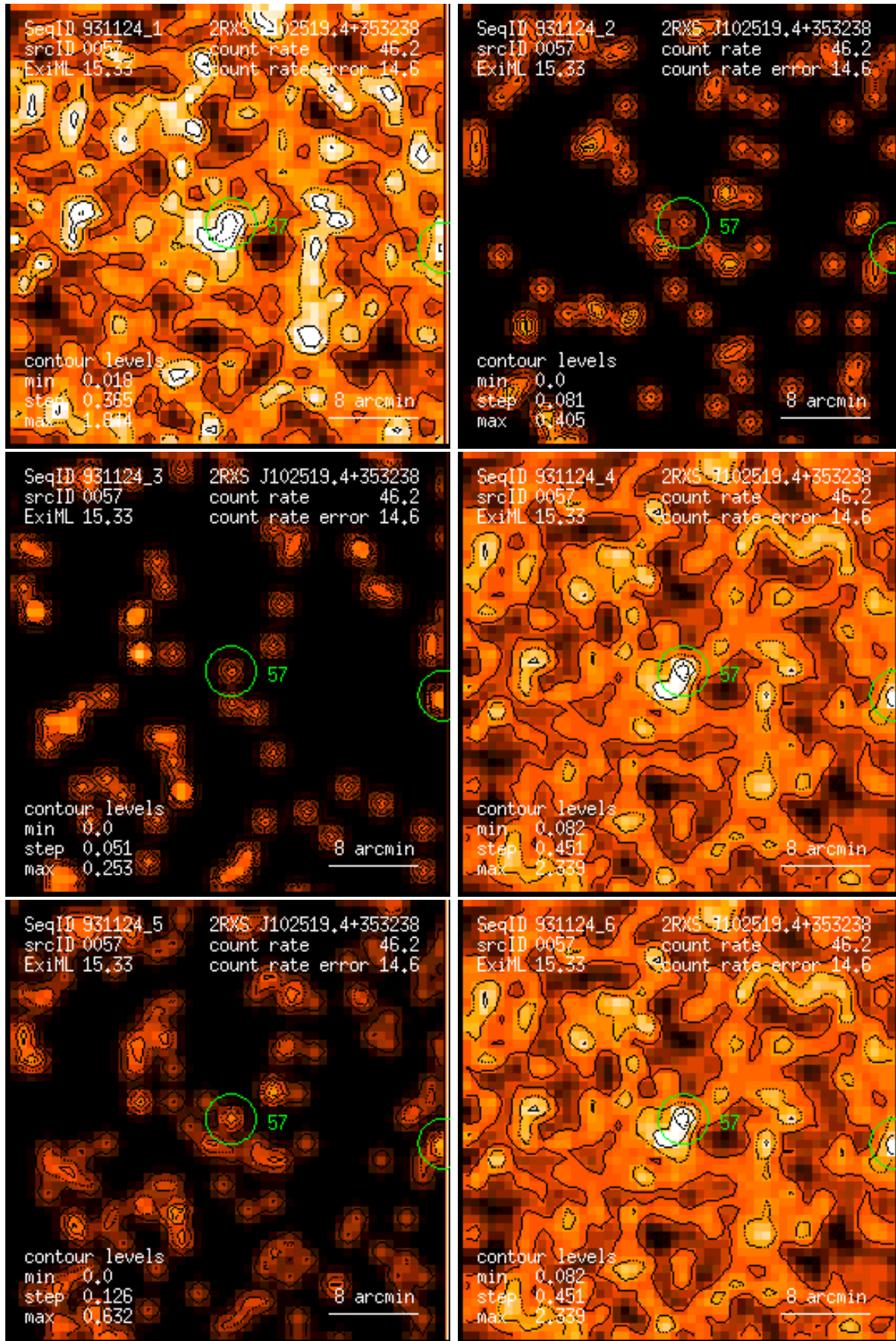
Figure 57: RASS 931124: detection 0057: band rate images, Gaussian filter: (1) PSPC channels 11 – 41, (2) 52 – 90, (3) 91 – 201, (4) 11 – 235, (5) 52 – 201, (6) 11 – 201. Broad band rates in counts/ks. Band rate contour levels in counts/ks/arcmin 2 .
