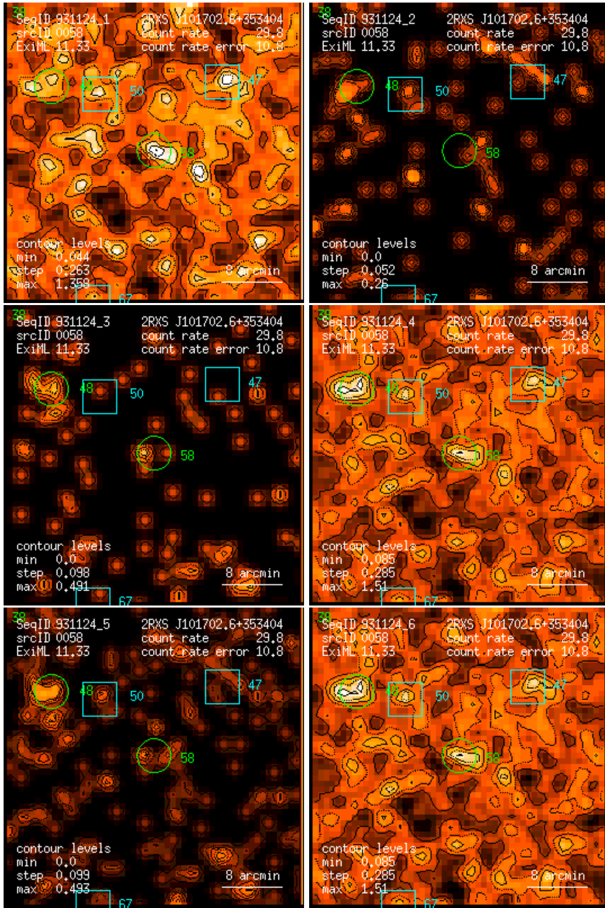
Figure 58: RASS 931124: detection 0058: band rate images, Gaussian filter: (1) PSPC channels 11 – 41, (2) 52 – 90, (3) 91 – 201, (4) 11 – 235, (5) 52 – 201, (6) 11 – 201. Broad band rates in counts/ks. Band rate contour levels in counts/ks/arcmin 2 .
