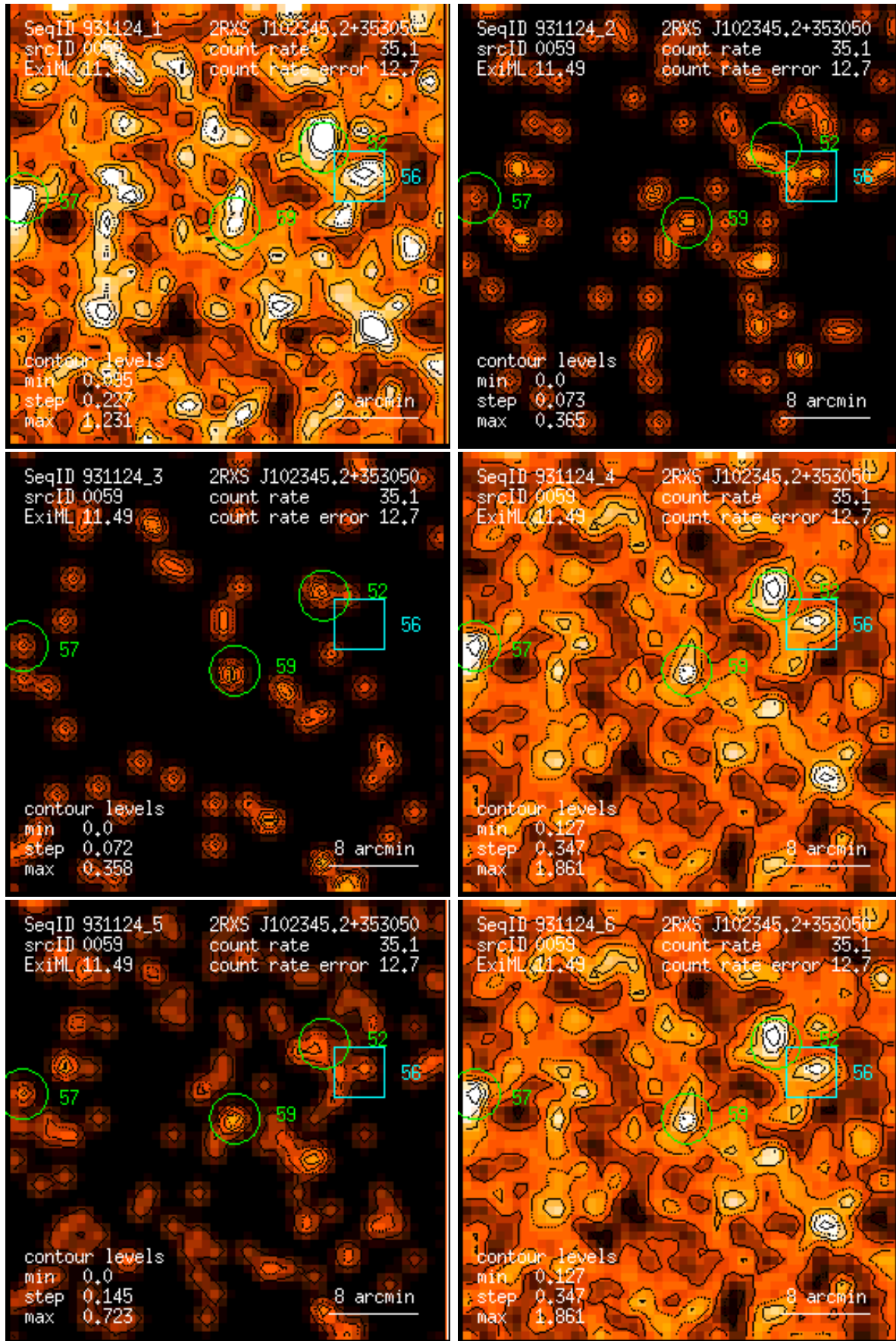
Figure 59: RASS 931124: detection 0059: band rate images, Gaussian filter: (1) PSPC channels 11 – 41, (2) 52 – 90, (3) 91 – 201, (4) 11 – 235, (5) 52 – 201, (6) 11 – 201. Broad band rates in counts/ks. Band rate contour levels in counts/ks/arcmin 2 .
