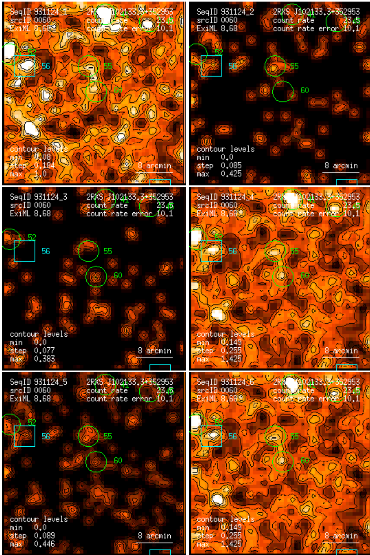
Figure 60: RASS 931124: detection 0060: band rate images, Gaussian filter: (1) PSPC channels 11 – 41, (2) 52 – 90, (3) 91 – 201, (4) 11 – 235, (5) 52 – 201, (6) 11 – 201. Broad band rates in counts/ks. Band rate contour levels in counts/ks/arcmin 2 .
