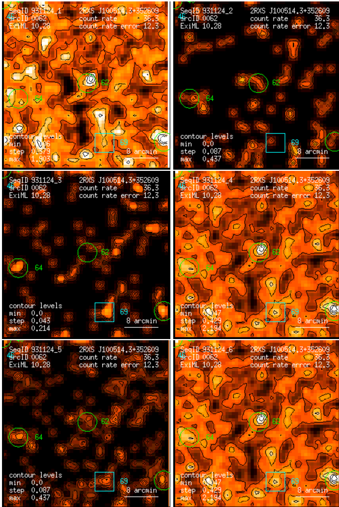
Figure 62: RASS 931124: detection 0062: band rate images, Gaussian filter: (1) PSPC channels 11 – 41, (2) 52 – 90, (3) 91 – 201, (4) 11 – 235, (5) 52 – 201, (6) 11 – 201. Broad band rates in counts/ks. Band rate contour levels in counts/ks/arcmin 2 .
