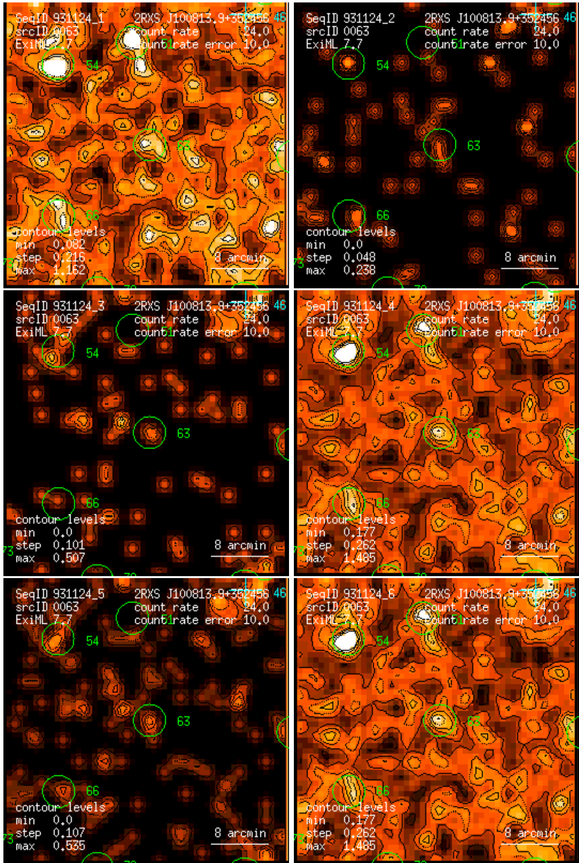
Figure 63: RASS 931124: detection 0063: band rate images, Gaussian filter: (1) PSPC channels 11 – 41, (2) 52 – 90, (3) 91 – 201, (4) 11 – 235, (5) 52 – 201, (6) 11 – 201. Broad band rates in counts/ks. Band rate contour levels in counts/ks/arcmin 2 .
