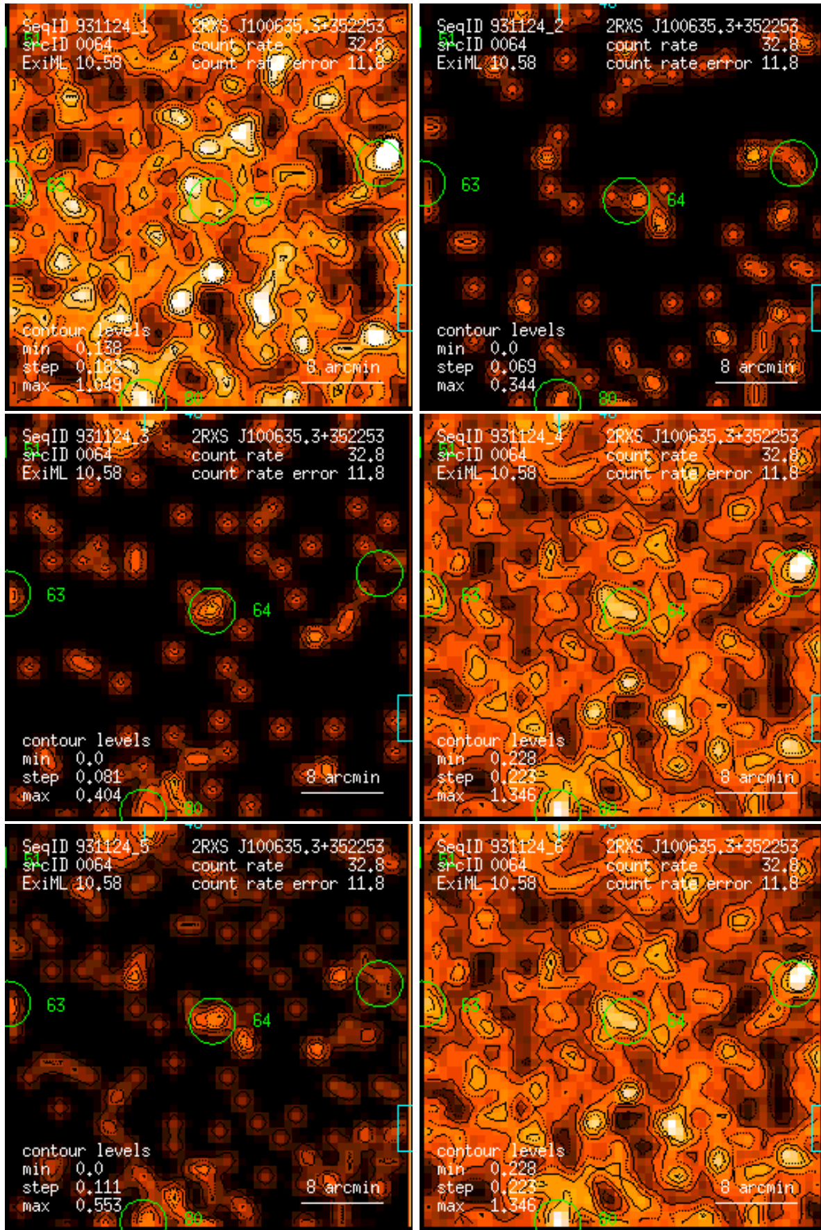
Figure 64: RASS 931124: detection 0064: band rate images, Gaussian filter: (1) PSPC channels 11 – 41, (2) 52 – 90, (3) 91 – 201, (4) 11 – 235, (5) 52 – 201, (6) 11 – 201. Broad band rates in counts/ks. Band rate contour levels in counts/ks/arcmin 2 .
