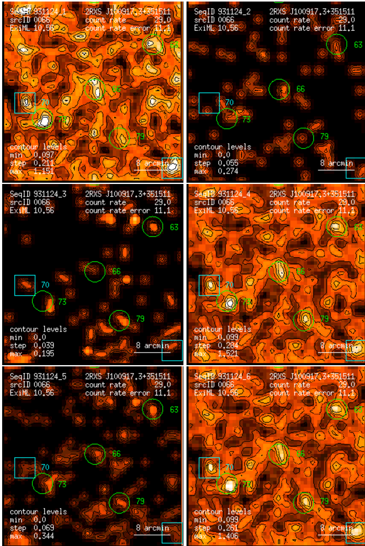
Figure 66: RASS 931124: detection 0066: band rate images, Gaussian filter: (1) PSPC channels 11 – 41, (2) 52 – 90, (3) 91 – 201, (4) 11 – 235, (5) 52 – 201, (6) 11 – 201. Broad band rates in counts/ks. Band rate contour levels in counts/ks/arcmin 2 .
