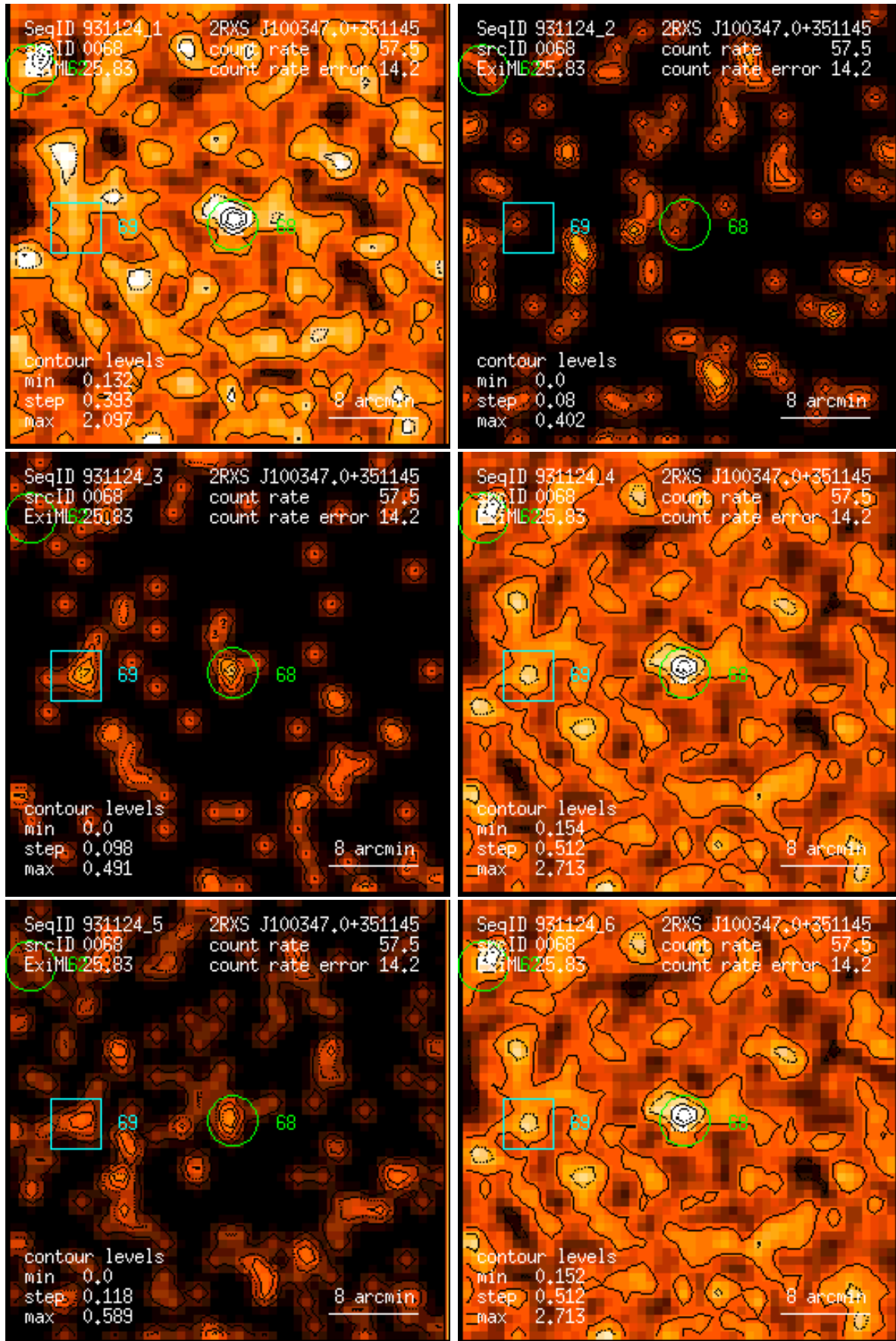
Figure 68: RASS 931124: detection 0068: band rate images, Gaussian filter: (1) PSPC channels 11 – 41, (2) 52 – 90, (3) 91 – 201, (4) 11 – 235, (5) 52 – 201, (6) 11 – 201. Broad band rates in counts/ks. Band rate contour levels in counts/ks/arcmin 2 .
