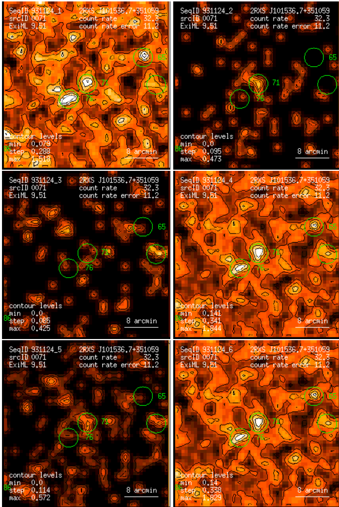
Figure 71: RASS 931124: detection 0071: band rate images, Gaussian filter: (1) PSPC channels 11 – 41, (2) 52 – 90, (3) 91 – 201, (4) 11 – 235, (5) 52 – 201, (6) 11 – 201. Broad band rates in counts/ks. Band rate contour levels in counts/ks/arcmin 2 .
