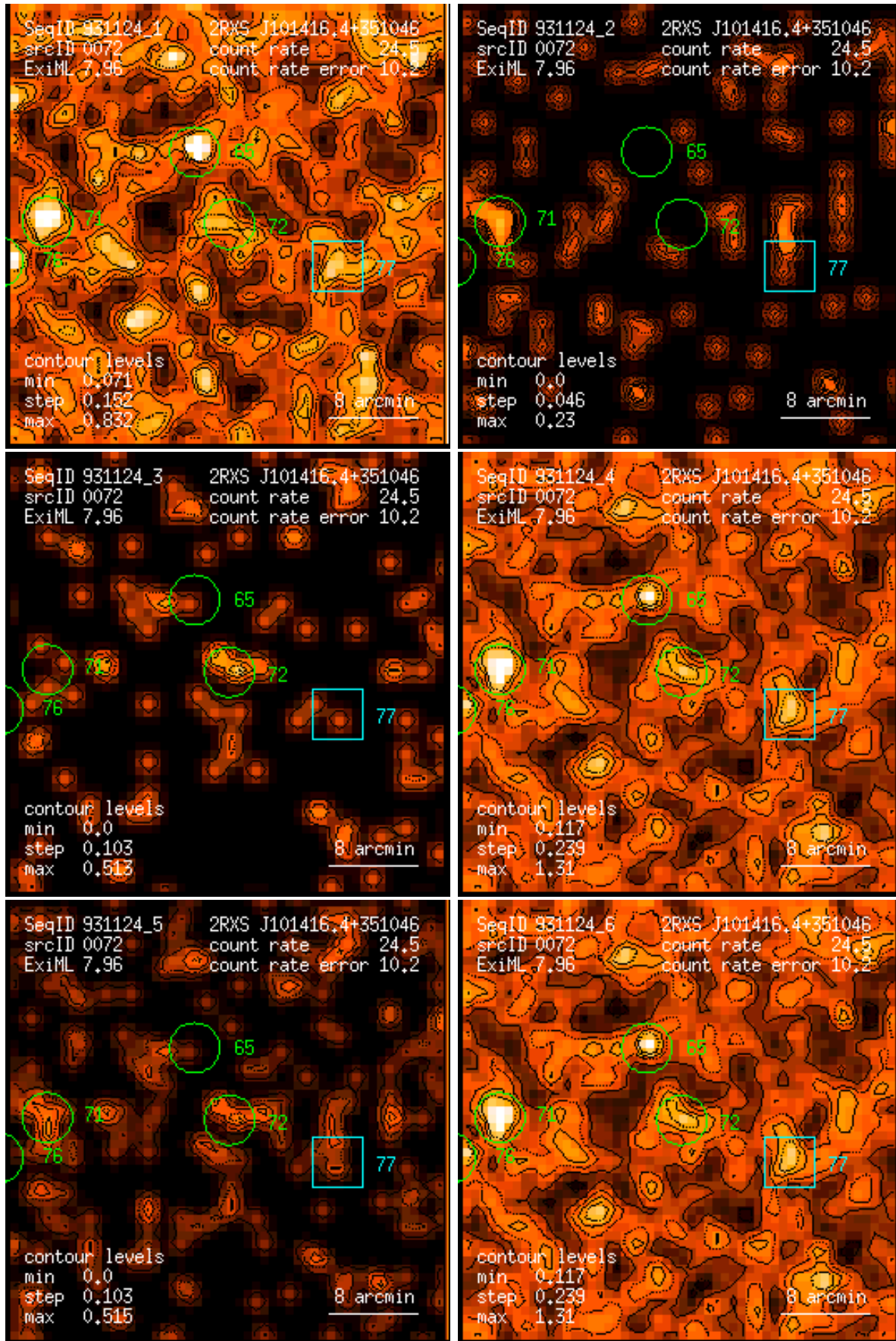
Figure 72: RASS 931124: detection 0072: band rate images, Gaussian filter: (1) PSPC channels 11 – 41, (2) 52 – 90, (3) 91 – 201, (4) 11 – 235, (5) 52 – 201, (6) 11 – 201. Broad band rates in counts/ks. Band rate contour levels in counts/ks/arcmin 2 .
