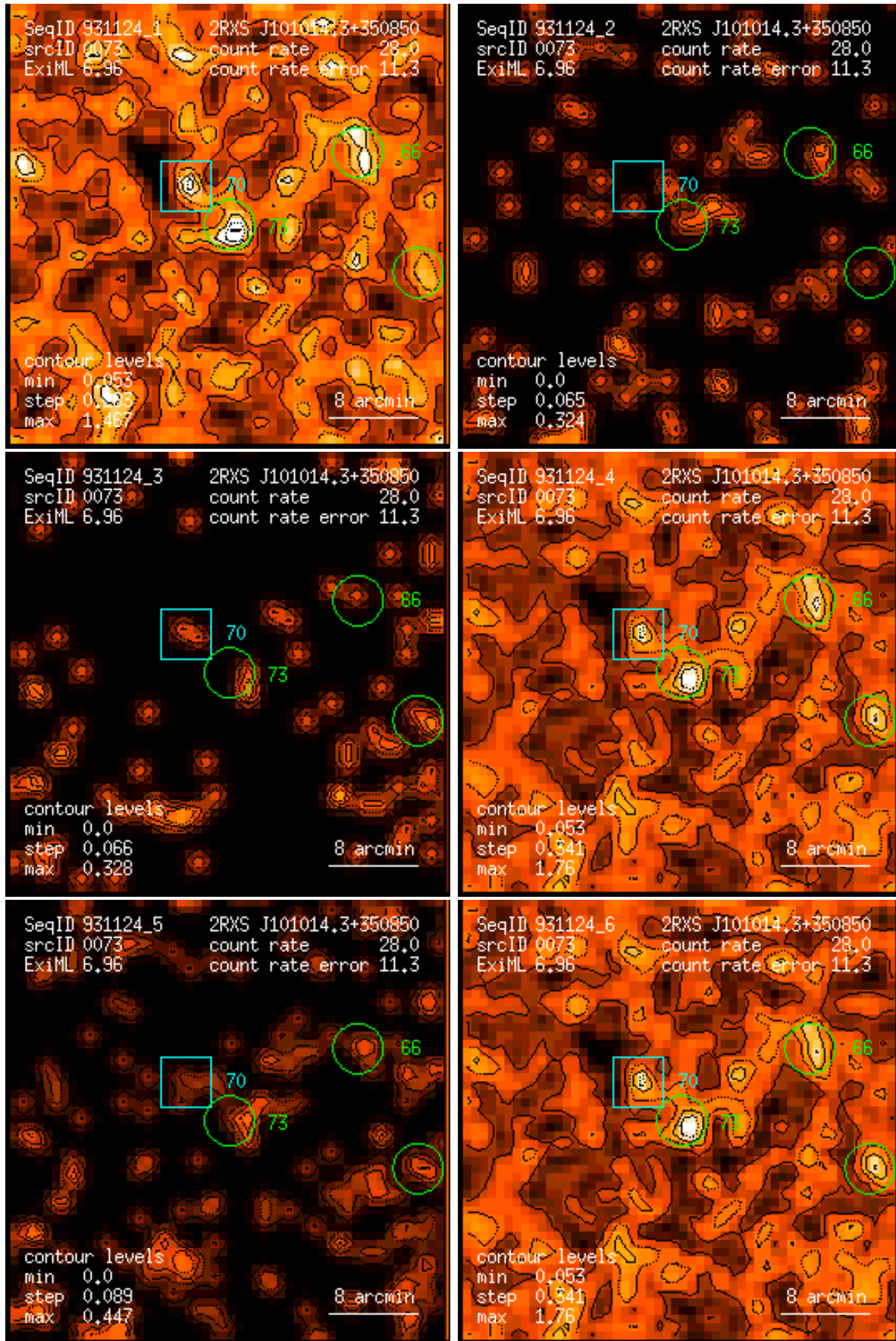
Figure 73: RASS 931124: detection 0073: band rate images, Gaussian filter: (1) PSPC channels 11 – 41, (2) 52 – 90, (3) 91 – 201, (4) 11 – 235, (5) 52 – 201, (6) 11 – 201. Broad band rates in counts/ks. Band rate contour levels in counts/ks/arcmin 2 .
