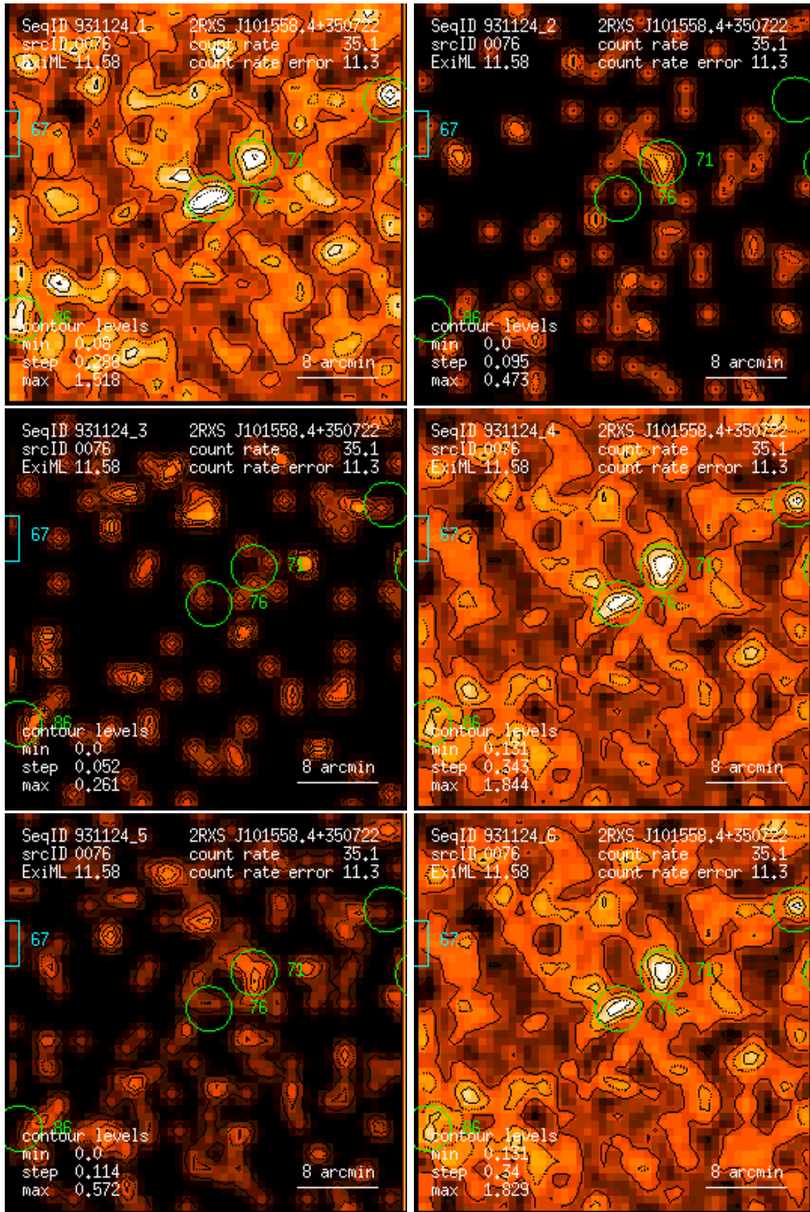
Figure 76: RASS 931124: detection 0076: band rate images, Gaussian filter: (1) PSPC channels 11 – 41, (2) 52 – 90, (3) 91 – 201, (4) 11 – 235, (5) 52 – 201, (6) 11 – 201. Broad band rates in counts/ks. Band rate contour levels in counts/ks/arcmin 2 .
