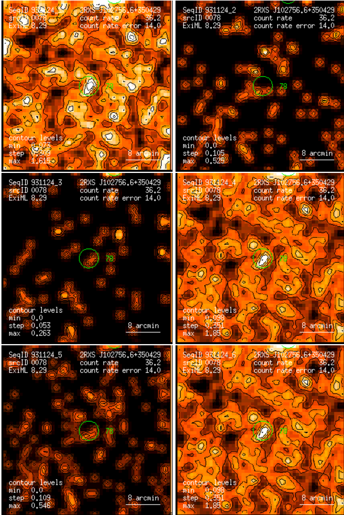
Figure 78: RASS 931124: detection 0078: band rate images, Gaussian filter: (1) PSPC channels 11 – 41, (2) 52 – 90, (3) 91 – 201, (4) 11 – 235, (5) 52 – 201, (6) 11 – 201. Broad band rates in counts/ks. Band rate contour levels in counts/ks/arcmin 2 .
