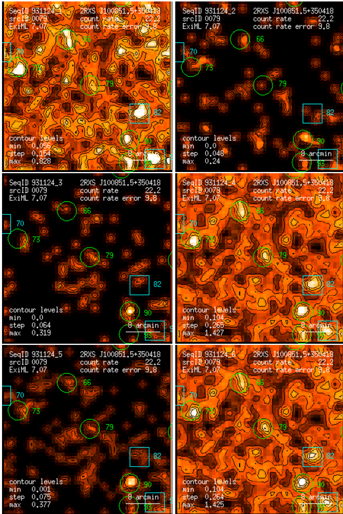
Figure 79: RASS 931124: detection 0079: band rate images, Gaussian filter: (1) PSPC channels 11 – 41, (2) 52 – 90, (3) 91 – 201, (4) 11 – 235, (5) 52 – 201, (6) 11 – 201. Broad band rates in counts/ks. Band rate contour levels in counts/ks/arcmin 2 .
