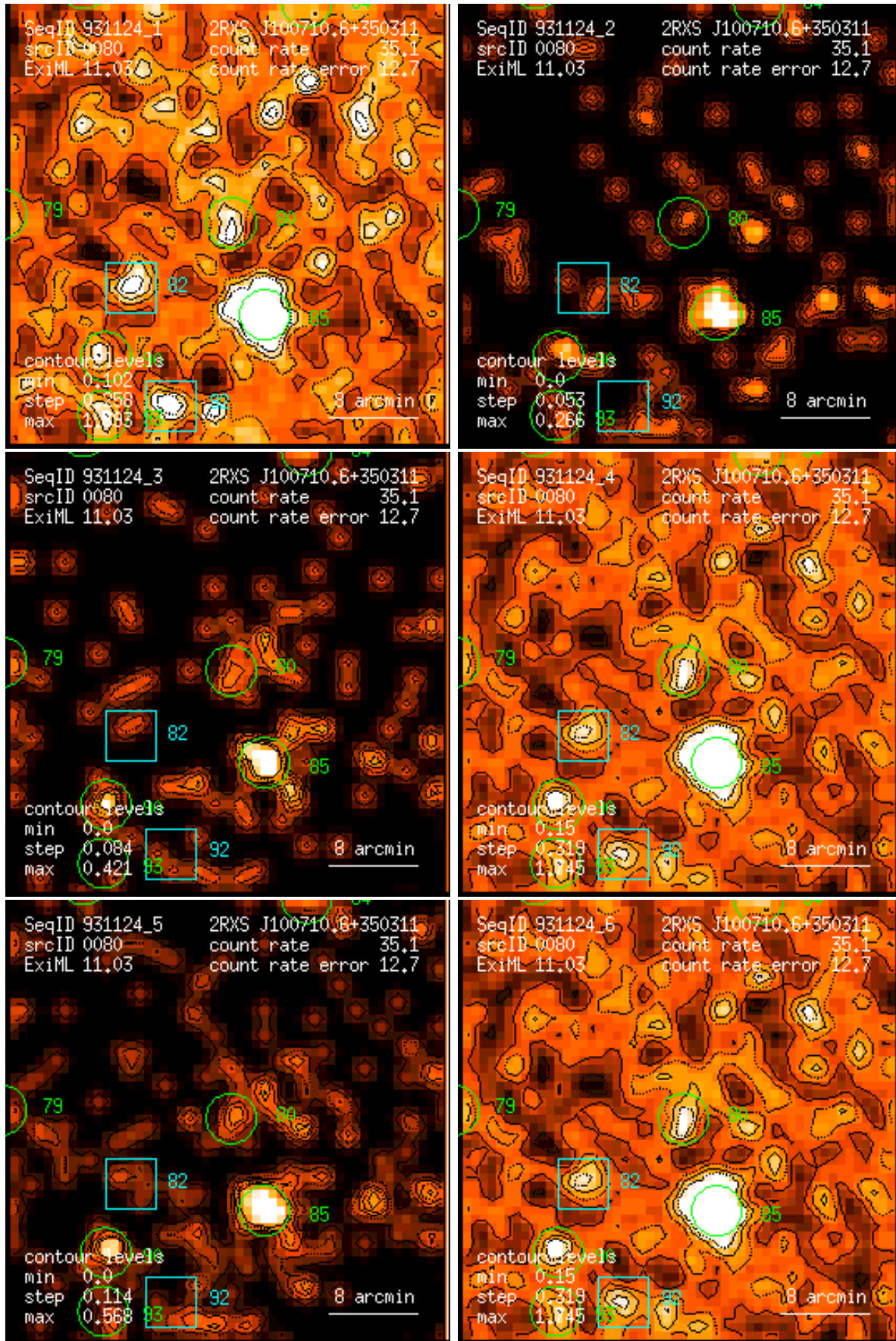
Figure 80: RASS 931124: detection 0080: band rate images, Gaussian filter: (1) PSPC channels 11 – 41, (2) 52 – 90, (3) 91 – 201, (4) 11 – 235, (5) 52 – 201, (6) 11 – 201. Broad band rates in counts/ks. Band rate contour levels in counts/ks/arcmin 2 .
