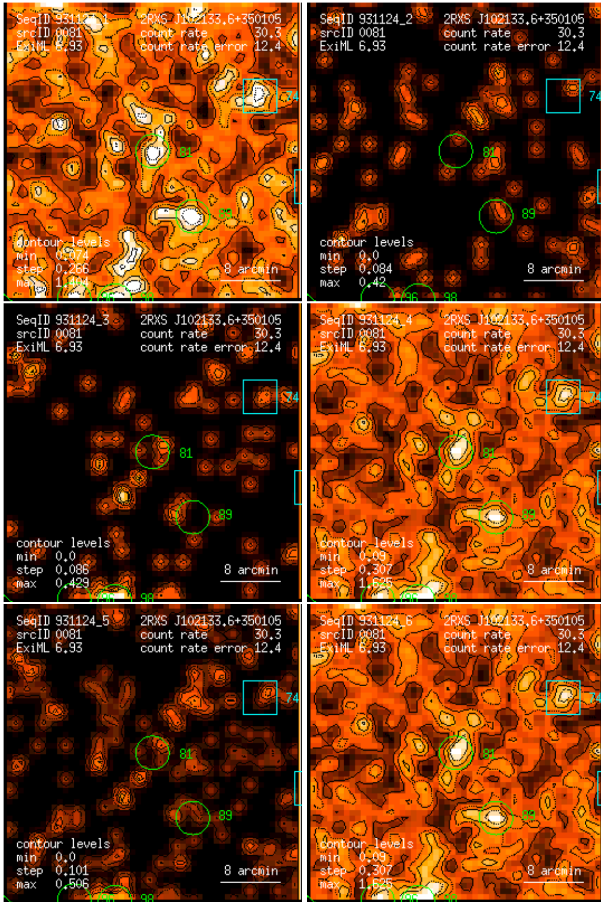
Figure 81: RASS 931124: detection 0081: band rate images, Gaussian filter: (1) PSPC channels 11 – 41, (2) 52 – 90, (3) 91 – 201, (4) 11 – 235, (5) 52 – 201, (6) 11 – 201. Broad band rates in counts/ks. Band rate contour levels in counts/ks/arcmin 2 .
