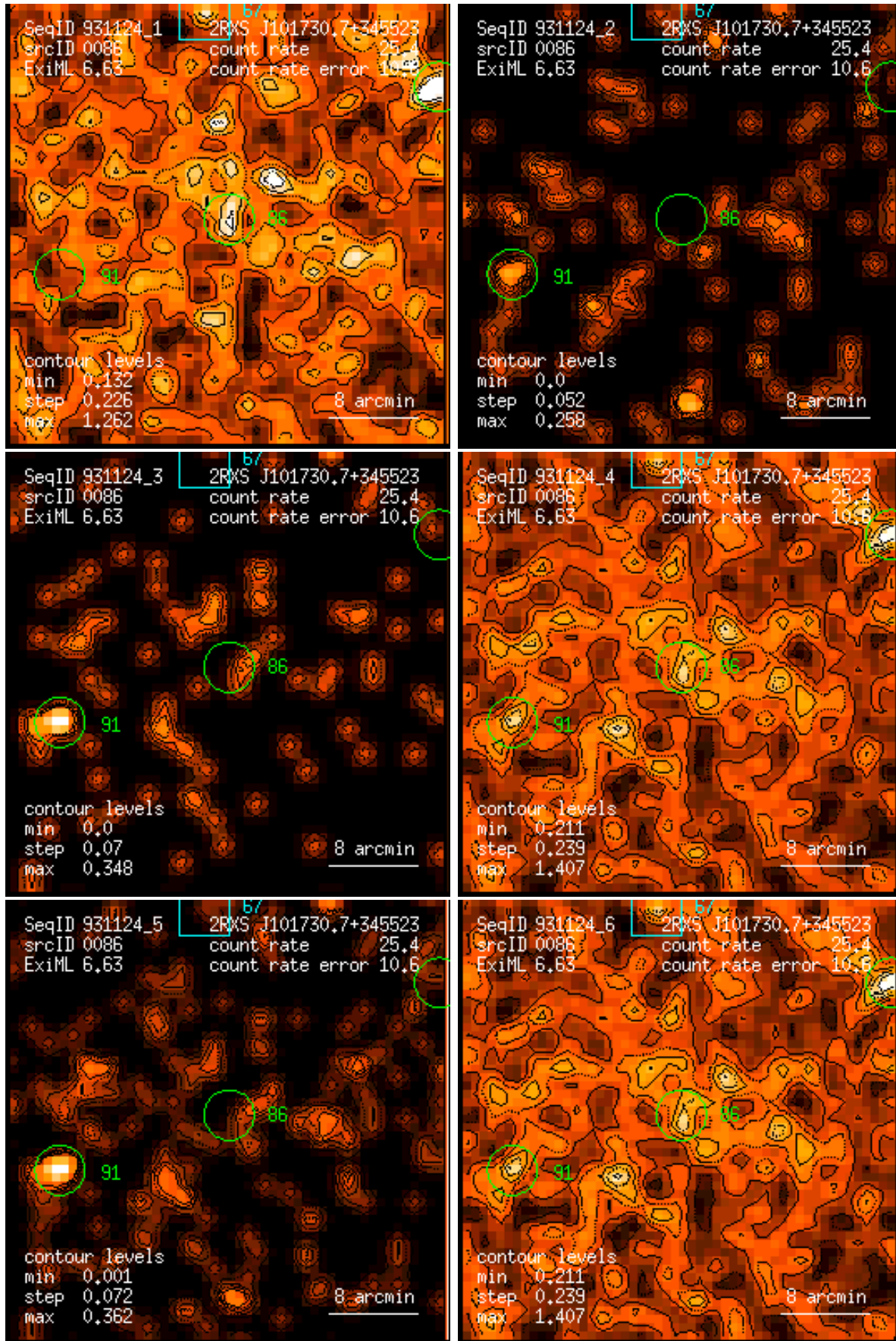
Figure 86: RASS 931124: detection 0086: band rate images, Gaussian filter: (1) PSPC channels 11 – 41, (2) 52 – 90, (3) 91 – 201, (4) 11 – 235, (5) 52 – 201, (6) 11 – 201. Broad band rates in counts/ks. Band rate contour levels in counts/ks/arcmin 2 .
