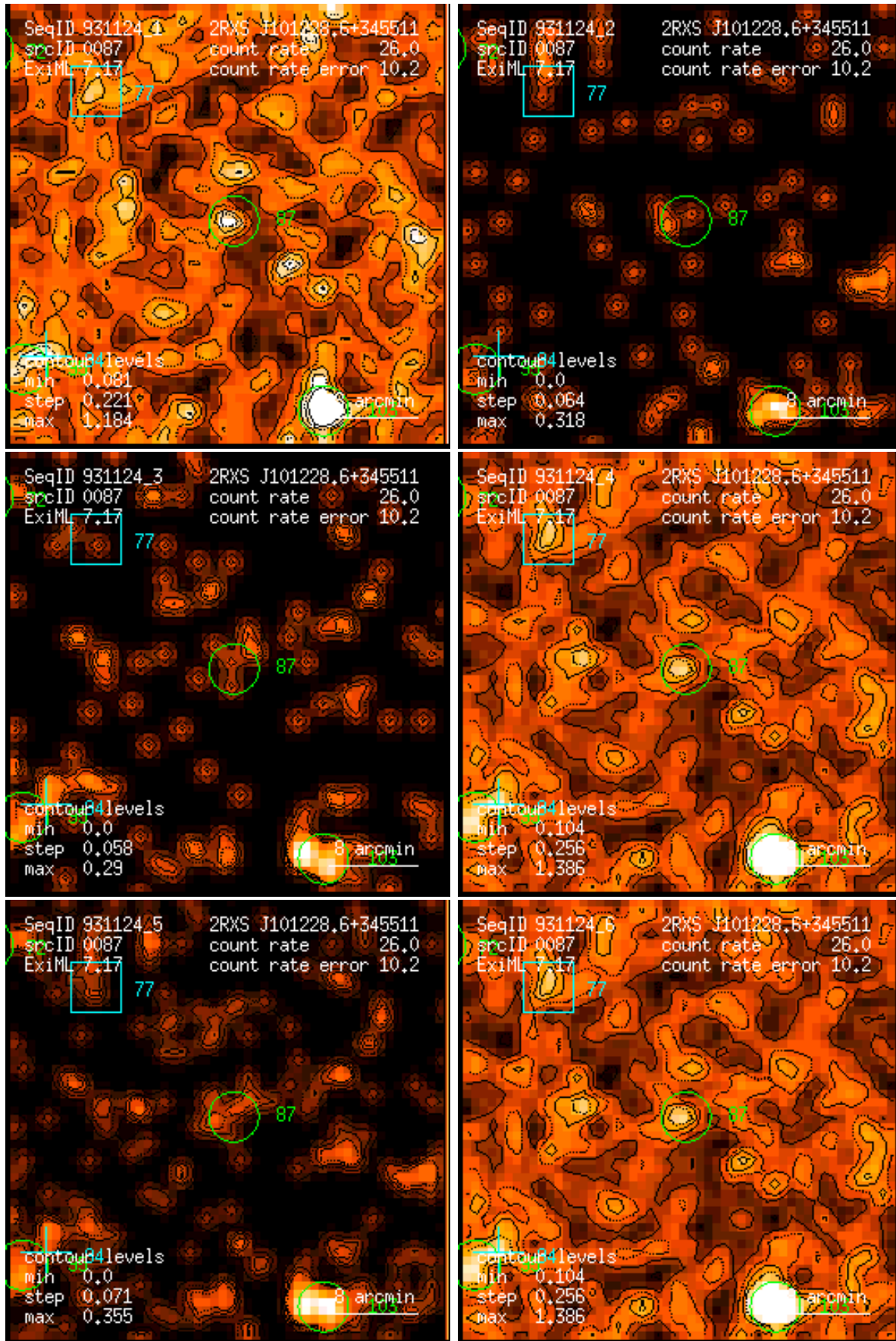
Figure 87: RASS 931124: detection 0087: band rate images, Gaussian filter: (1) PSPC channels 11 – 41, (2) 52 – 90, (3) 91 – 201, (4) 11 – 235, (5) 52 – 201, (6) 11 – 201. Broad band rates in counts/ks. Band rate contour levels in counts/ks/arcmin 2 .
