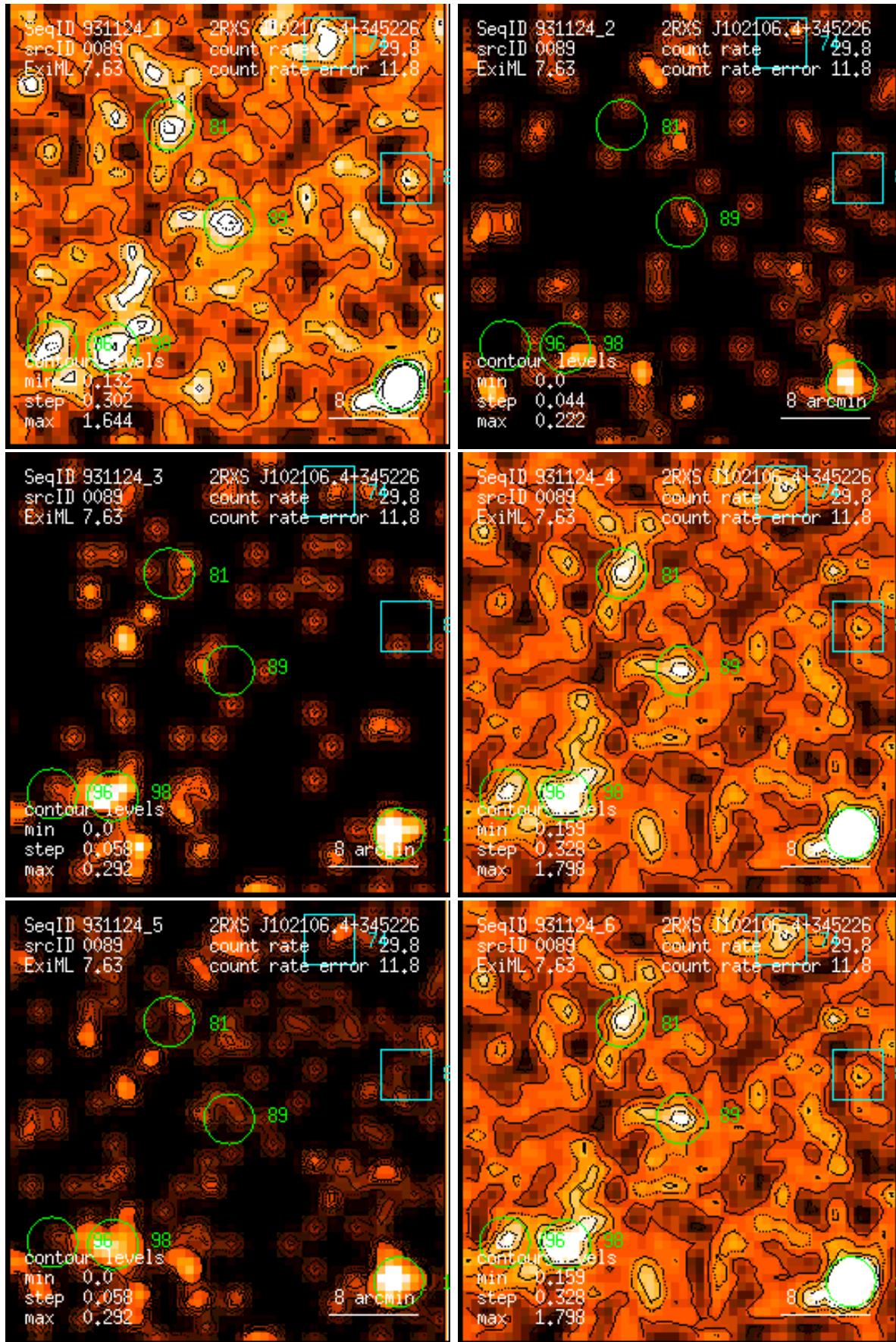
Figure 89: RASS 931124: detection 0089: band rate images, Gaussian filter: (1) PSPC channels 11 – 41, (2) 52 – 90, (3) 91 – 201, (4) 11 – 235, (5) 52 – 201, (6) 11 – 201. Broad band rates in counts/ks. Band rate contour levels in counts/ks/arcmin 2 .
