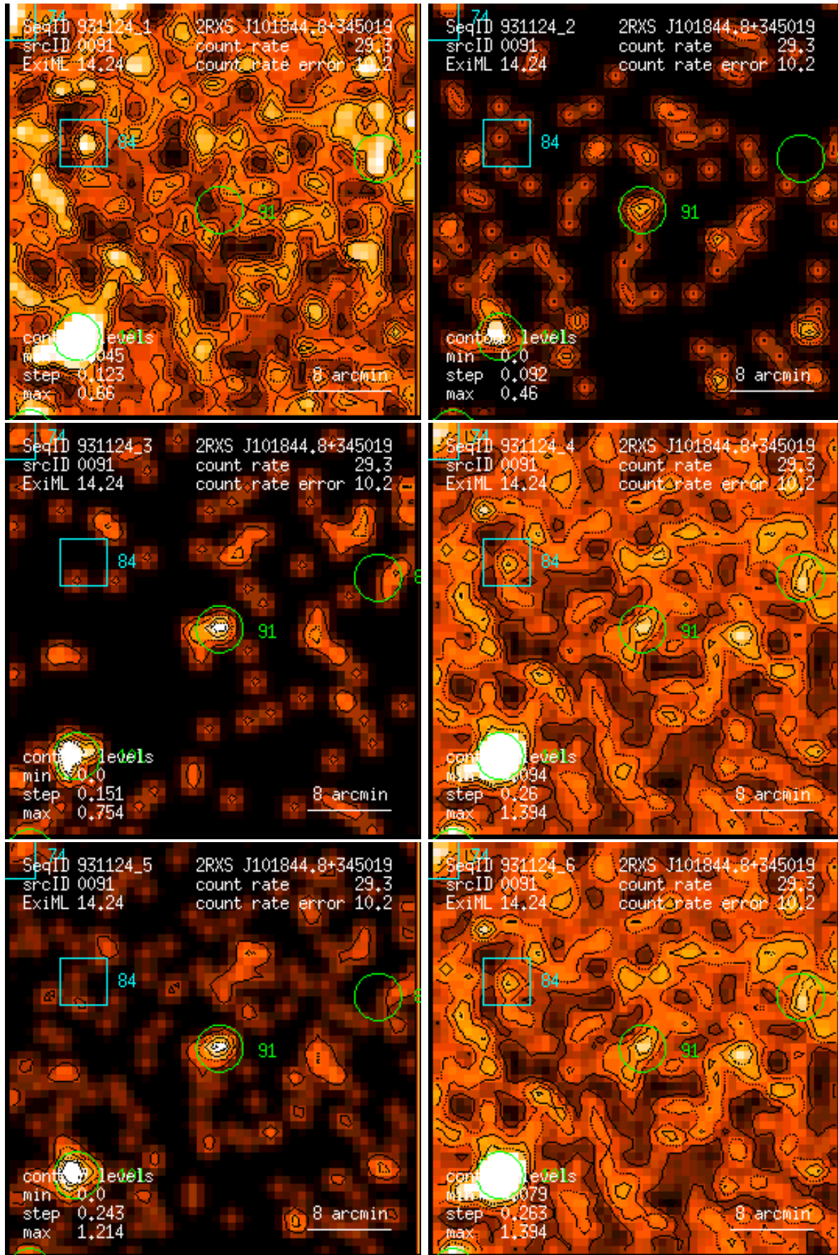
Figure 91: RASS 931124: detection 0091: band rate images, Gaussian filter: (1) PSPC channels 11 – 41, (2) 52 – 90, (3) 91 – 201, (4) 11 – 235, (5) 52 – 201, (6) 11 – 201. Broad band rates in counts/ks. Band rate contour levels in counts/ks/arcmin 2 .
