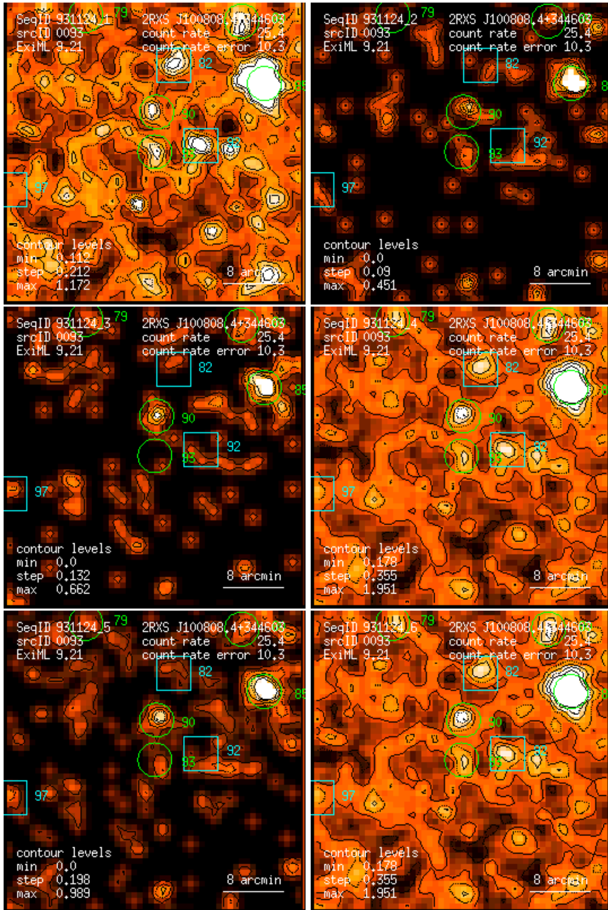
Figure 93: RASS 931124: detection 0093: band rate images, Gaussian filter: (1) PSPC channels 11 – 41, (2) 52 – 90, (3) 91 – 201, (4) 11 – 235, (5) 52 – 201, (6) 11 – 201. Broad band rates in counts/ks. Band rate contour levels in counts/ks/arcmin 2 .
