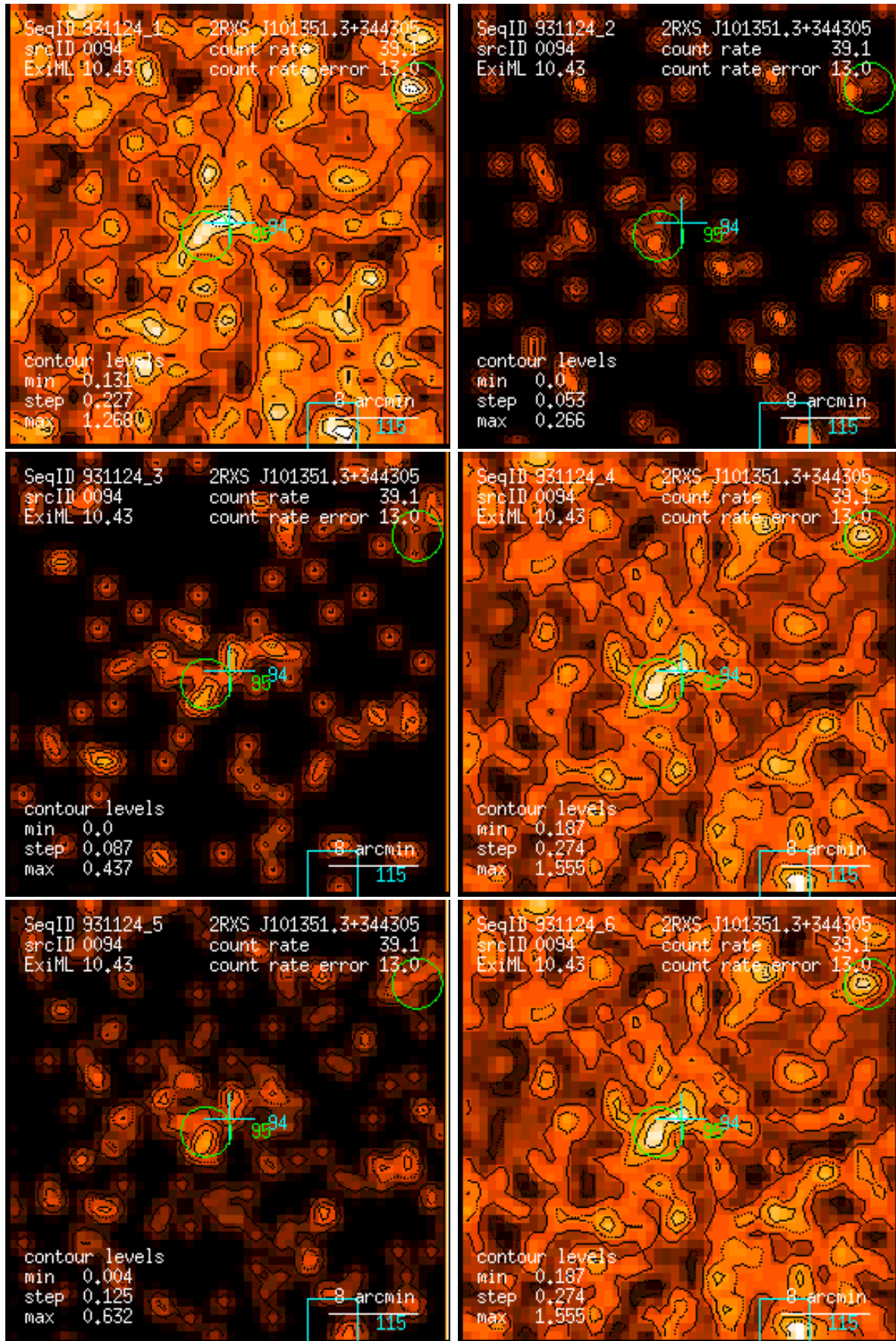
Figure 94: RASS 931124: detection 0094: band rate images, Gaussian filter: (1) PSPC channels 11 – 41, (2) 52 – 90, (3) 91 – 201, (4) 11 – 235, (5) 52 – 201, (6) 11 – 201. Broad band rates in counts/ks. Band rate contour levels in counts/ks/arcmin 2 .
