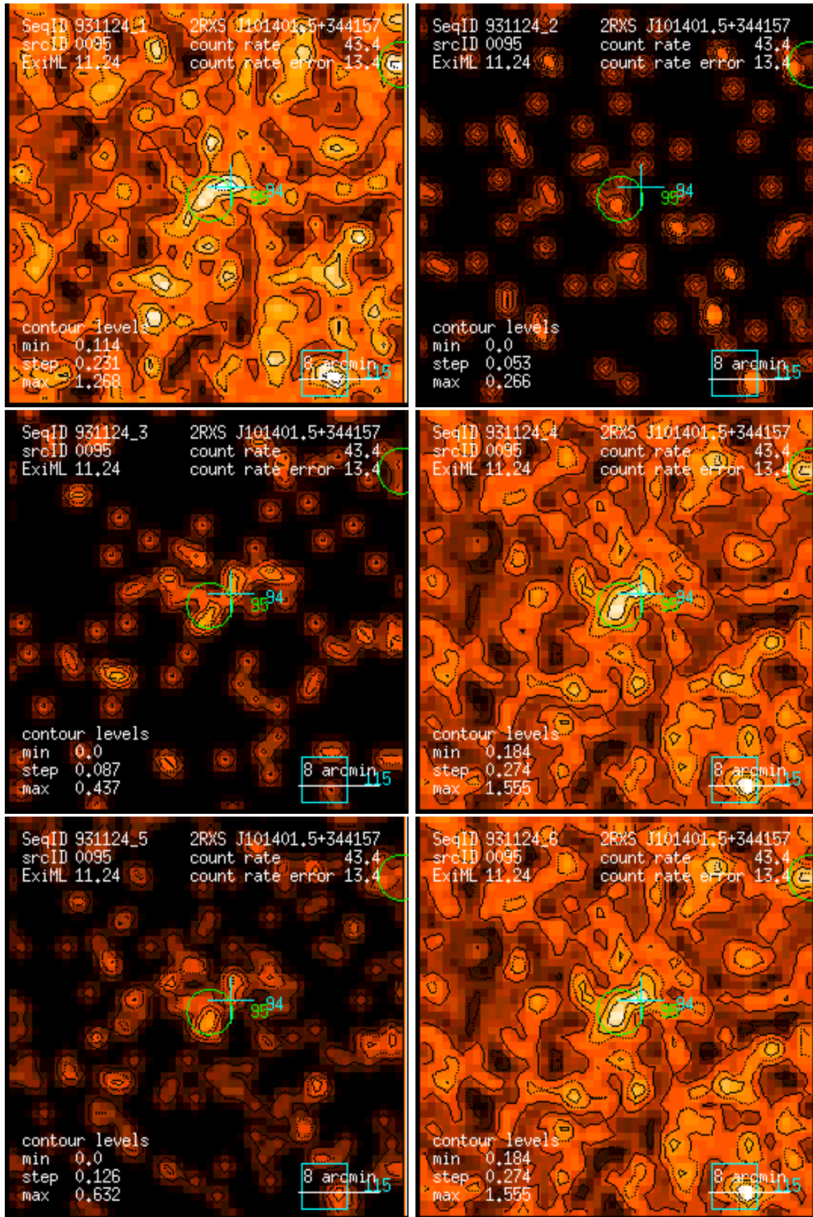
Figure 95: RASS 931124: detection 0095: band rate images, Gaussian filter: (1) PSPC channels 11 – 41, (2) 52 – 90, (3) 91 – 201, (4) 11 – 235, (5) 52 – 201, (6) 11 – 201. Broad band rates in counts/ks. Band rate contour levels in counts/ks/arcmin 2 .
