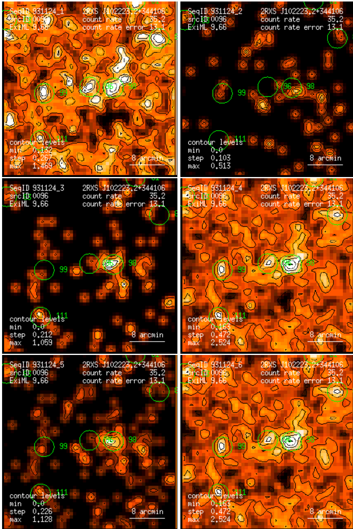
Figure 96: RASS 931124: detection 0096: band rate images, Gaussian filter: (1) PSPC channels 11 – 41, (2) 52 – 90, (3) 91 – 201, (4) 11 – 235, (5) 52 – 201, (6) 11 – 201. Broad band rates in counts/ks. Band rate contour levels in counts/ks/arcmin 2 .
