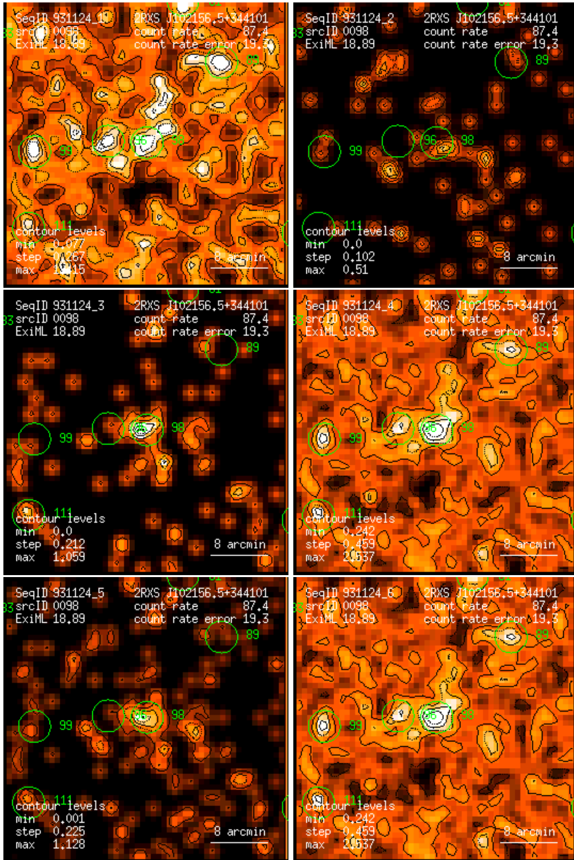
Figure 98: RASS 931124: detection 0098: band rate images, Gaussian filter: (1) PSPC channels 11 – 41, (2) 52 – 90, (3) 91 – 201, (4) 11 – 235, (5) 52 – 201, (6) 11 – 201. Broad band rates in counts/ks. Band rate contour levels in counts/ks/arcmin 2 .
