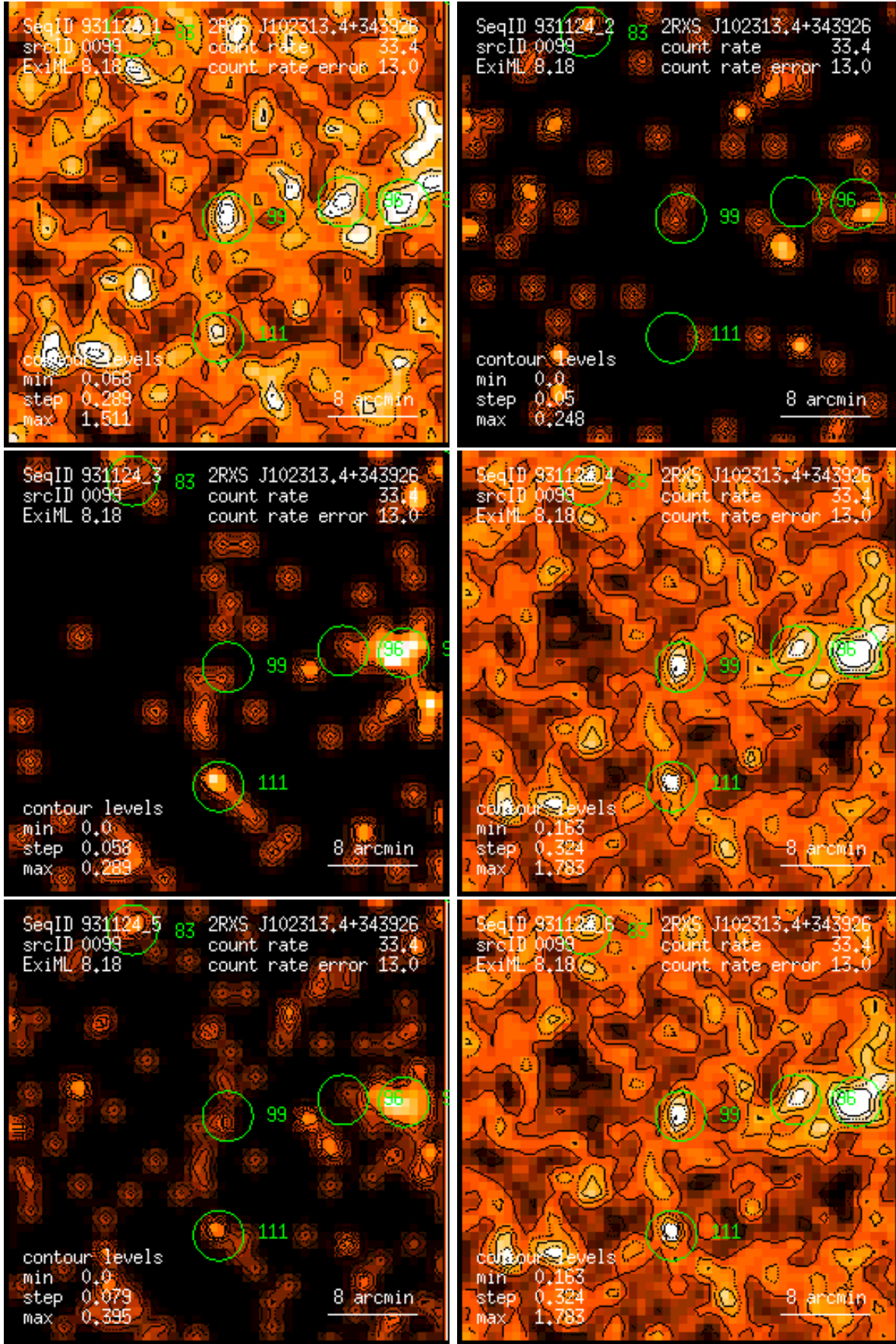
Figure 99: RASS 931124: detection 0099: band rate images, Gaussian filter: (1) PSPC channels 11 – 41, (2) 52 – 90, (3) 91 – 201, (4) 11 – 235, (5) 52 – 201, (6) 11 – 201. Broad band rates in counts/ks. Band rate contour levels in counts/ks/arcmin 2 .
