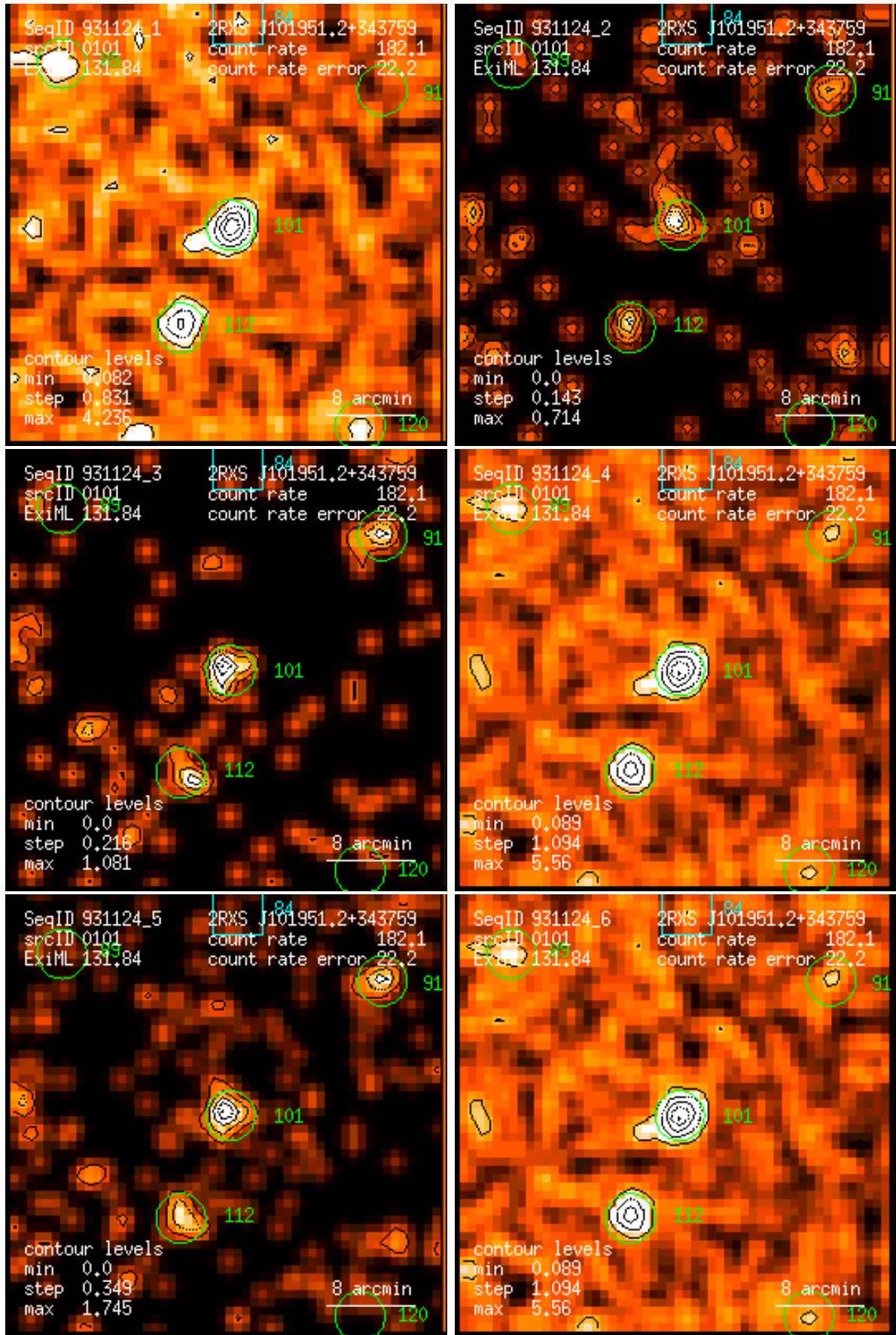
Figure 101: RASS 931124: detection 0101: band rate images, Gaussian filter: (1) PSPC channels 11 – 41, (2) 52 – 90, (3) 91 – 201, (4) 11 – 235, (5) 52 – 201, (6) 11 – 201. Broad band rates in counts/ks. Band rate contour levels in counts/ks/arcmin 2 .
