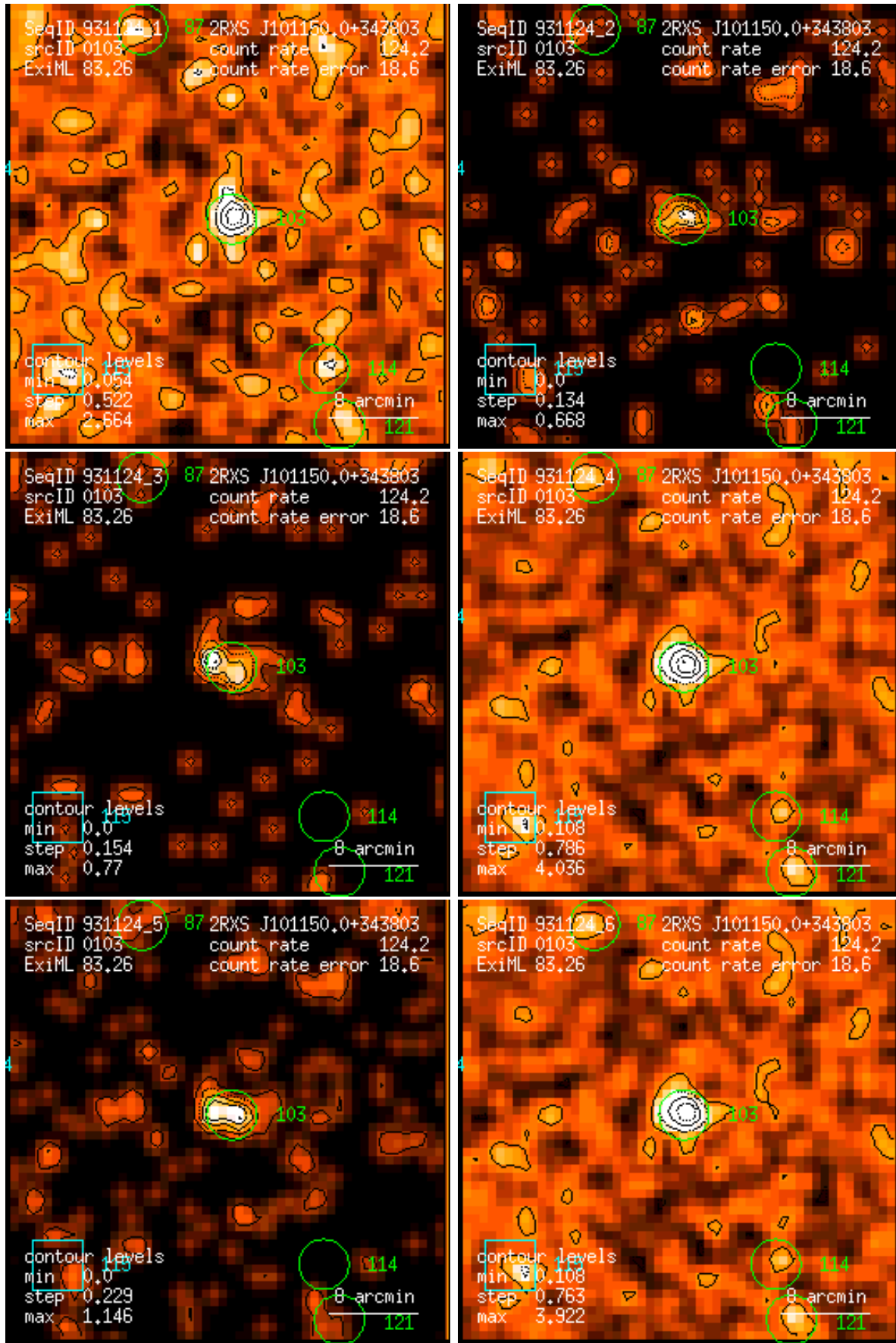
Figure 103: RASS 931124: detection 0103: band rate images, Gaussian filter: (1) PSPC channels 11 – 41, (2) 52 – 90, (3) 91 – 201, (4) 11 – 235, (5) 52 – 201, (6) 11 – 201. Broad band rates in counts/ks. Band rate contour levels in counts/ks/arcmin 2 .
