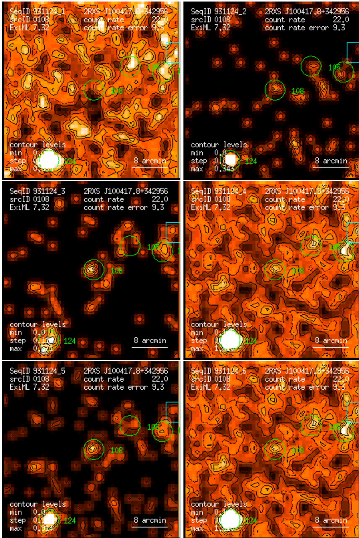
Figure 108: RASS 931124: detection 0108: band rate images, Gaussian filter: (1) PSPC channels 11 – 41, (2) 52 – 90, (3) 91 – 201, (4) 11 – 235, (5) 52 – 201, (6) 11 – 201. Broad band rates in counts/ks. Band rate contour levels in counts/ks/arcmin 2 .
