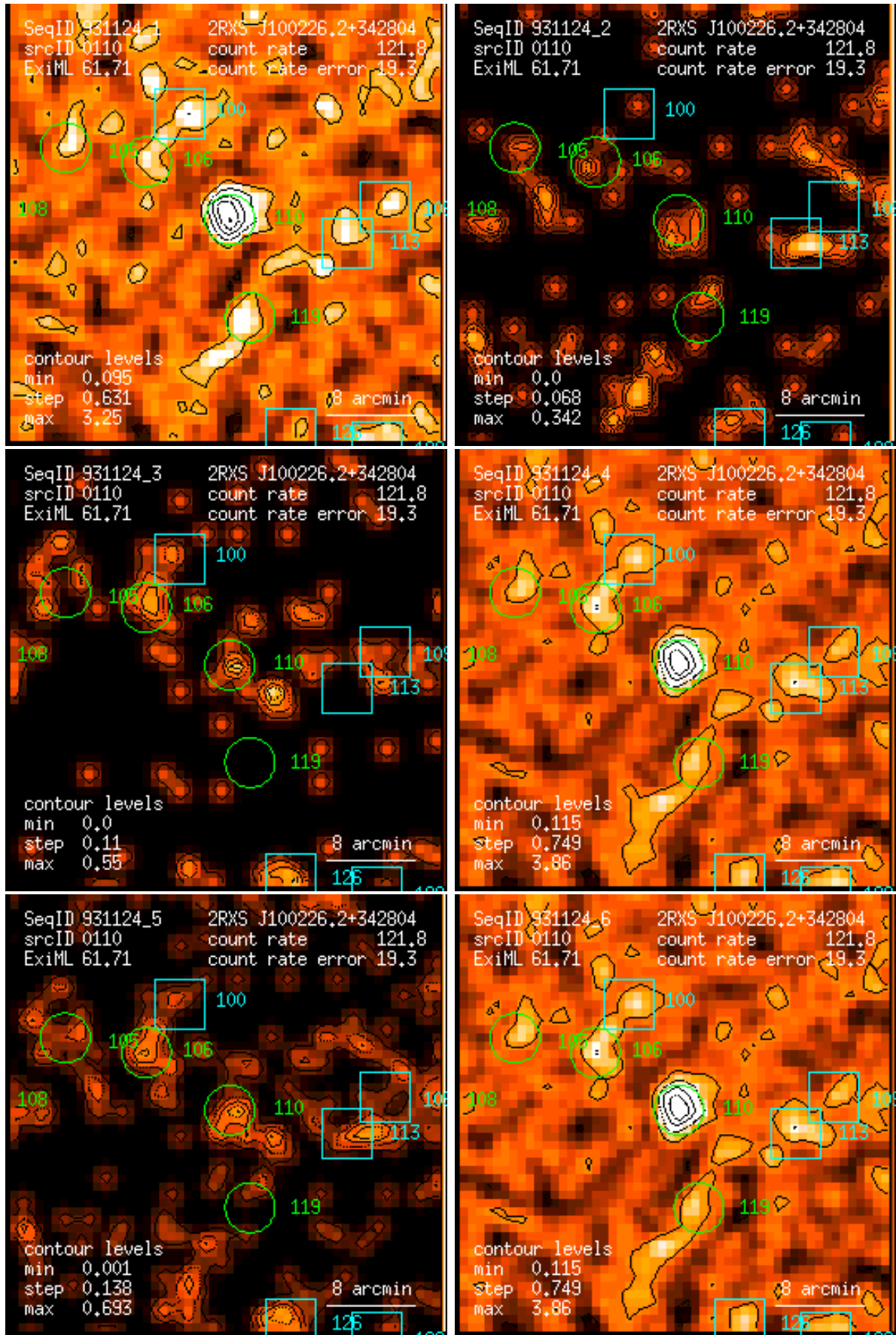
Figure 110: RASS 931124: detection 0110: band rate images, Gaussian filter: (1) PSPC channels 11 – 41, (2) 52 – 90, (3) 91 – 201, (4) 11 – 235, (5) 52 – 201, (6) 11 – 201. Broad band rates in counts/ks. Band rate contour levels in counts/ks/arcmin 2 .
