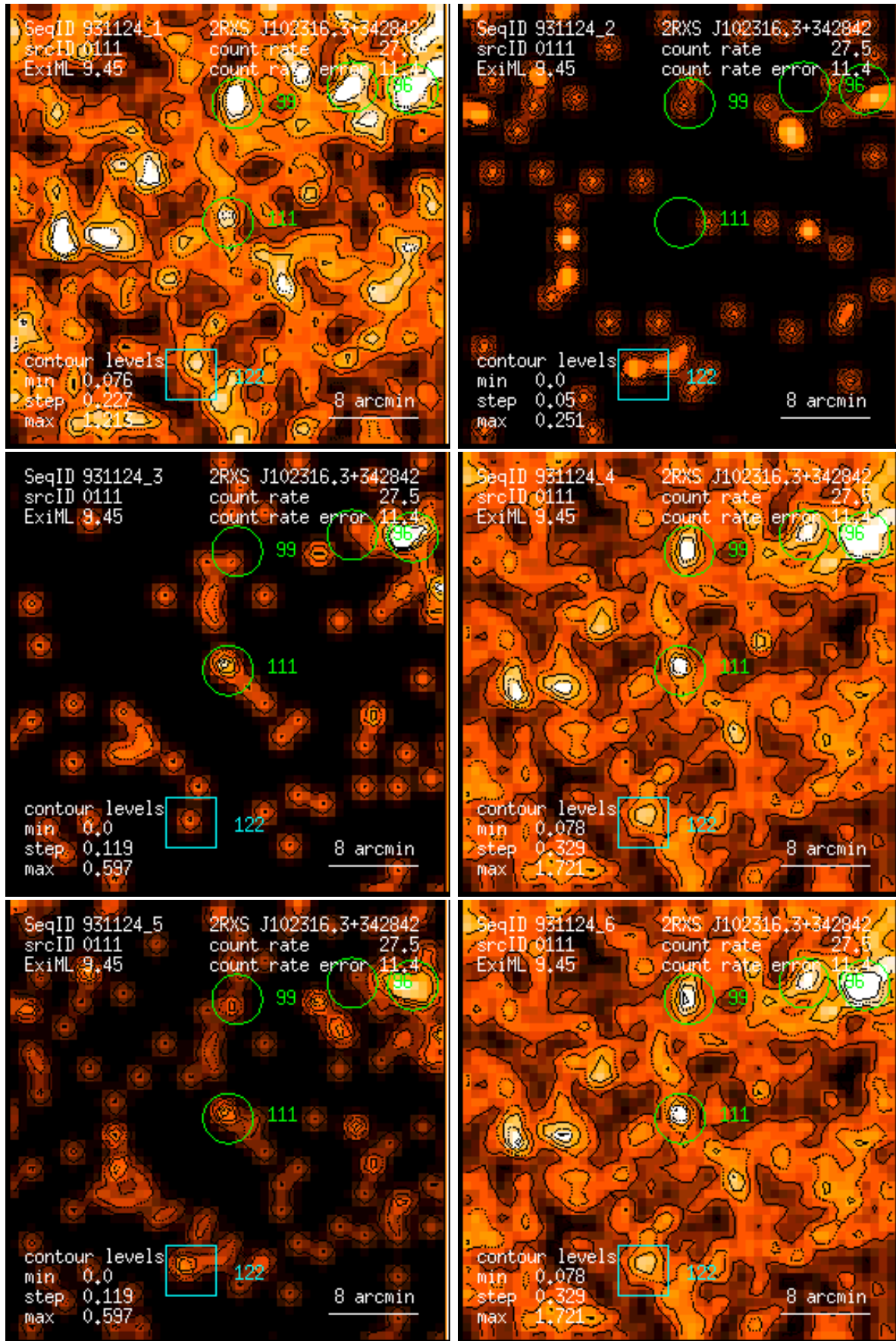
Figure 111: RASS 931124: detection 0111: band rate images, Gaussian filter: (1) PSPC channels 11 – 41, (2) 52 – 90, (3) 91 – 201, (4) 11 – 235, (5) 52 – 201, (6) 11 – 201. Broad band rates in counts/ks. Band rate contour levels in counts/ks/arcmin 2 .
