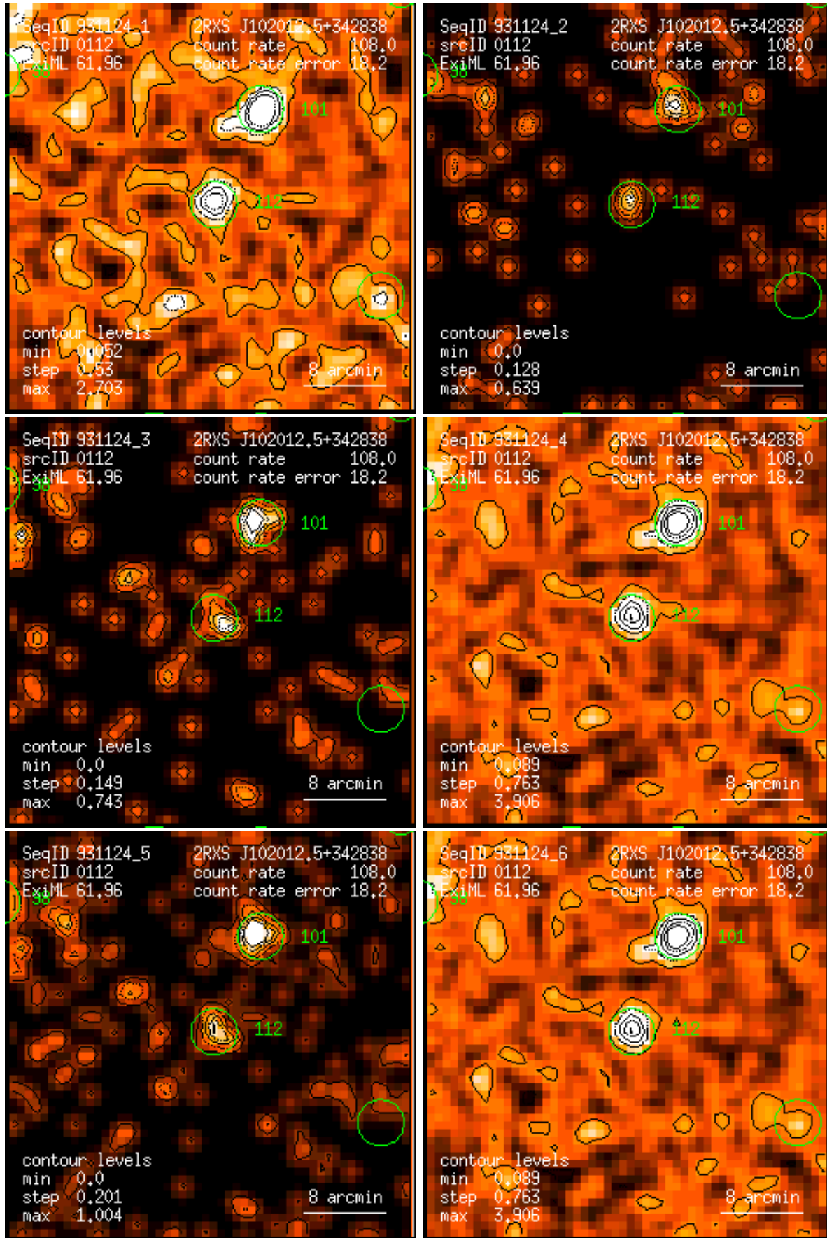
Figure 112: RASS 931124: detection 0112: band rate images, Gaussian filter: (1) PSPC channels 11 – 41, (2) 52 – 90, (3) 91 – 201, (4) 11 – 235, (5) 52 – 201, (6) 11 – 201. Broad band rates in counts/ks. Band rate contour levels in counts/ks/arcmin 2 .
