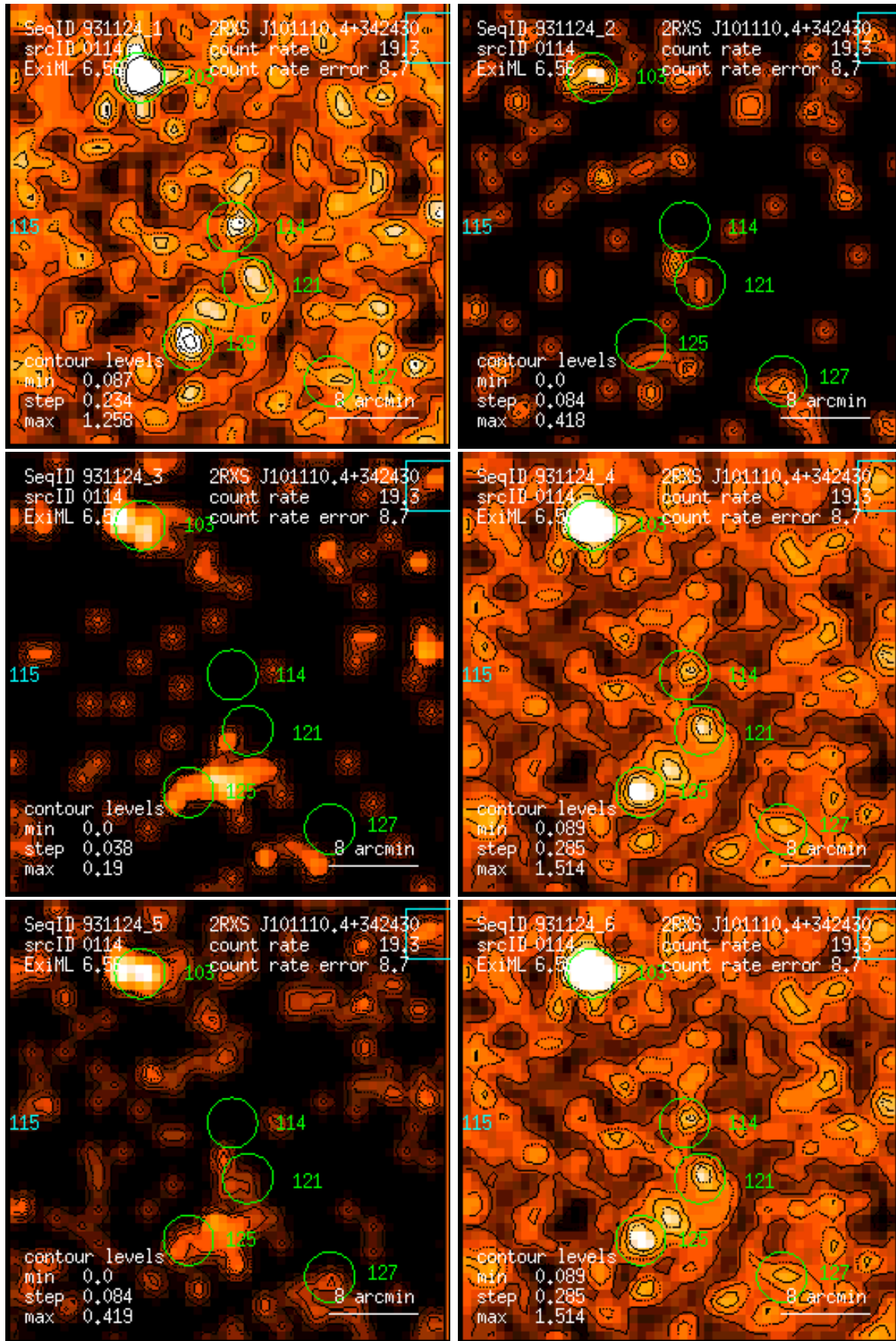
Figure 114: RASS 931124: detection 0114: band rate images, Gaussian filter: (1) PSPC channels 11 – 41, (2) 52 – 90, (3) 91 – 201, (4) 11 – 235, (5) 52 – 201, (6) 11 – 201. Broad band rates in counts/ks. Band rate contour levels in counts/ks/arcmin 2 .
