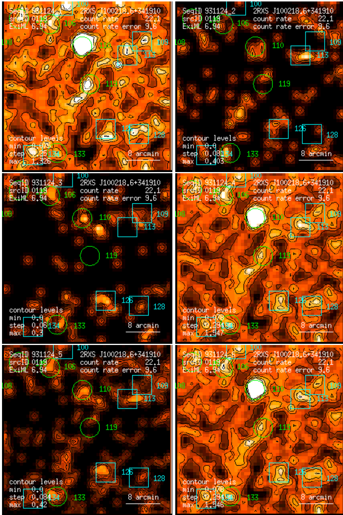
Figure 119: RASS 931124: detection 0119: band rate images, Gaussian filter: (1) PSPC channels 11 – 41, (2) 52 – 90, (3) 91 – 201, (4) 11 – 235, (5) 52 – 201, (6) 11 – 201. Broad band rates in counts/ks. Band rate contour levels in counts/ks/arcmin 2 .
