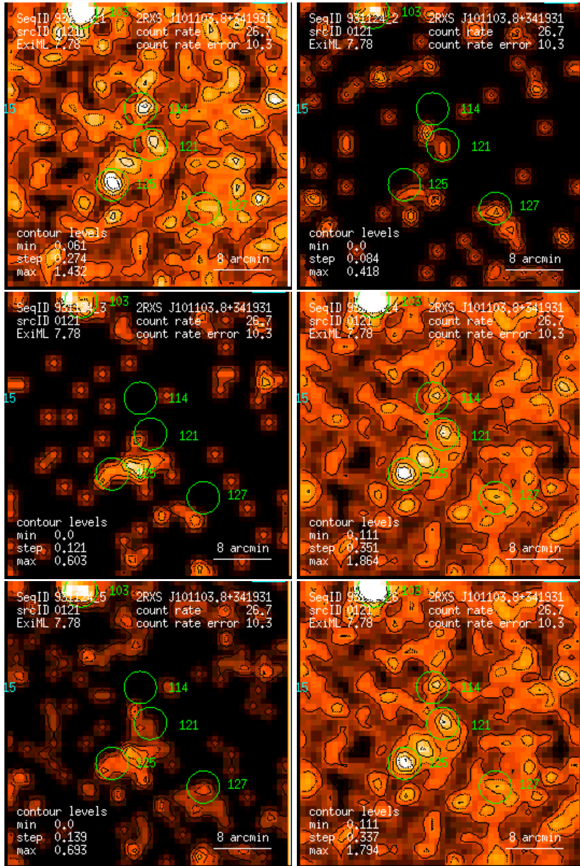
Figure 121: RASS 931124: detection 0121: band rate images, Gaussian filter: (1) PSPC channels 11 – 41, (2) 52 – 90, (3) 91 – 201, (4) 11 – 235, (5) 52 – 201, (6) 11 – 201. Broad band rates in counts/ks. Band rate contour levels in counts/ks/arcmin 2 .
