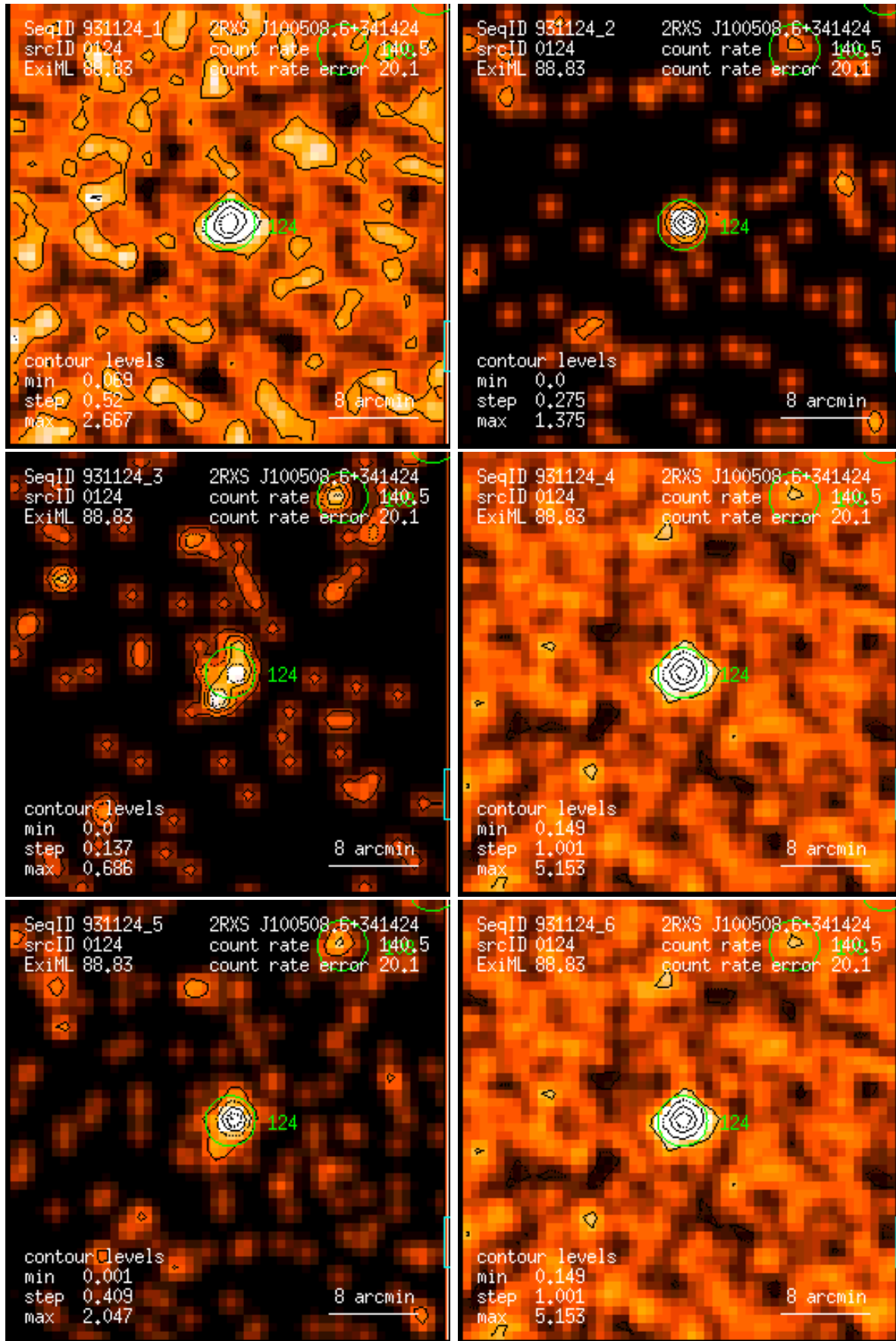
Figure 124: RASS 931124: detection 0124: band rate images, Gaussian filter: (1) PSPC channels 11 – 41, (2) 52 – 90, (3) 91 – 201, (4) 11 – 235, (5) 52 – 201, (6) 11 – 201. Broad band rates in counts/ks. Band rate contour levels in counts/ks/arcmin 2 .
